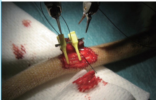
Fig. 7. Rat nerve model
