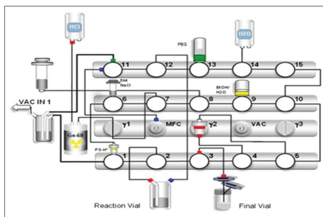
Figure 2: Schematic automated procedures for synthesis of 68 Ga-prostate-specific membrane antigen-11
