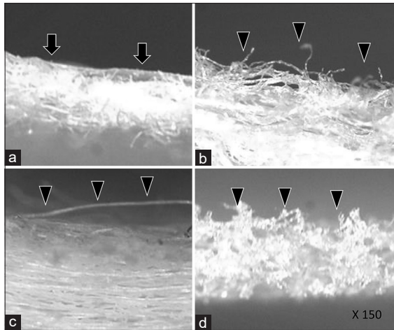
Figure 3: Transverse sections of four different surgical patties were investigated by light microscopy (magnification \times 150 ). Non-Stina X ® did not show any fluffing (a, arrow) on the polyurethane-coated surface. However, the other types of surgical patties, (b-d) showed some fluffing on their surfaces
