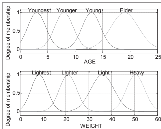
Figure 3: Membership functions for two inputs - patient age (AGE) and weight (WEIGHT)
