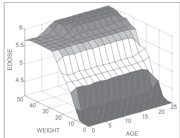
Figure 5: The surfaces between inputs and outputs
