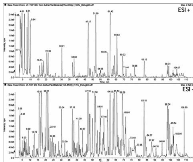
Fig. 1 TIC of cycloartane and flavonoid glycosides from stem-leaves of Sutherlandia frutescens by using HPLC-ESI-MSD-TOF.
