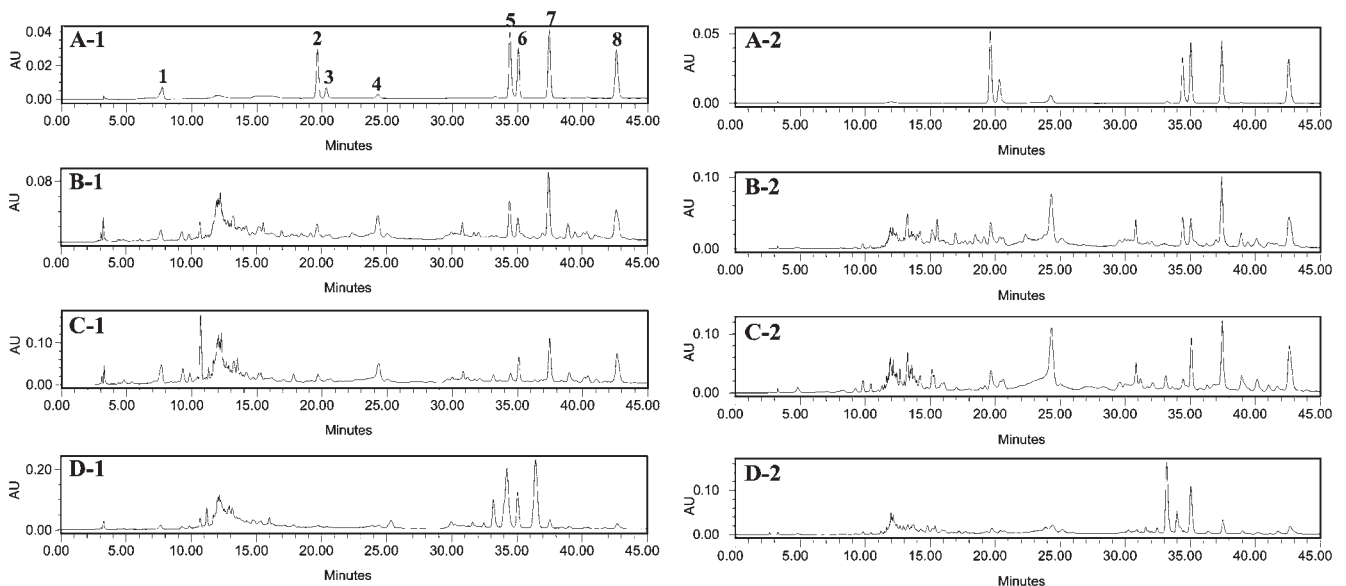
Fig. 1 HPLC-UV chromatograms of a standard mix. (A), extracts of T. diffusa . (B) and dietary supplements (C–D) at wavelength 280 nm (1) and 345 nm (2).
