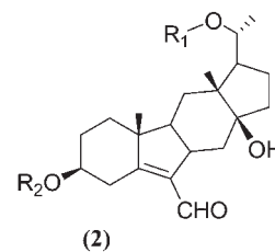
R 2 : β-(4-O-tigloyl)-D-thevetopyranosyl-(1→4)-β-D-oleandropyranoside
