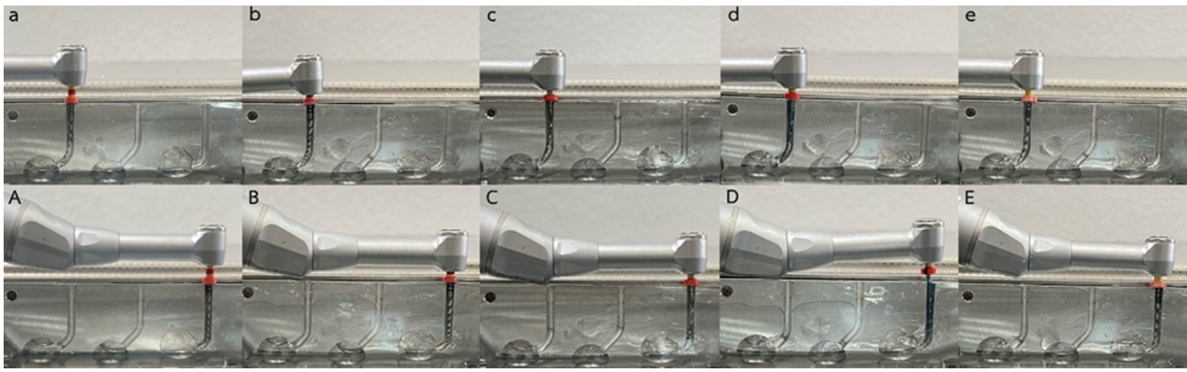
Fig. 1 Schematic of cyclic fatigue testing device adapted from Phumpatrakom et al. 10 Nickel-titanium (NiTi) rotary instruments in an artificial 60-degree curvature canal (upper row) and 90-degree curvature canal (lower row). NiTi rotary instruments were immersed in 37°C water bath: (a, A) ProTaper Universal, (b, B) ProTaper Next, (c, C) E-FLEX EDGE, (d, D) E-FLEX ONE, and (e, E) ZenFlex.
