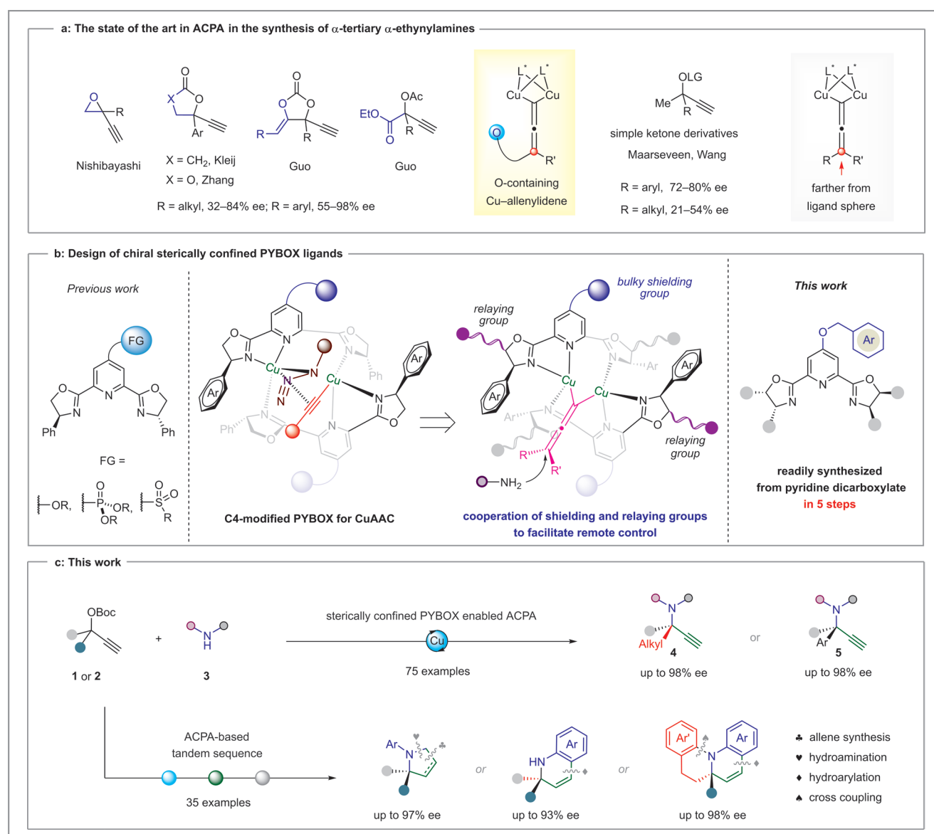
Scheme 1 Working hypothesis
