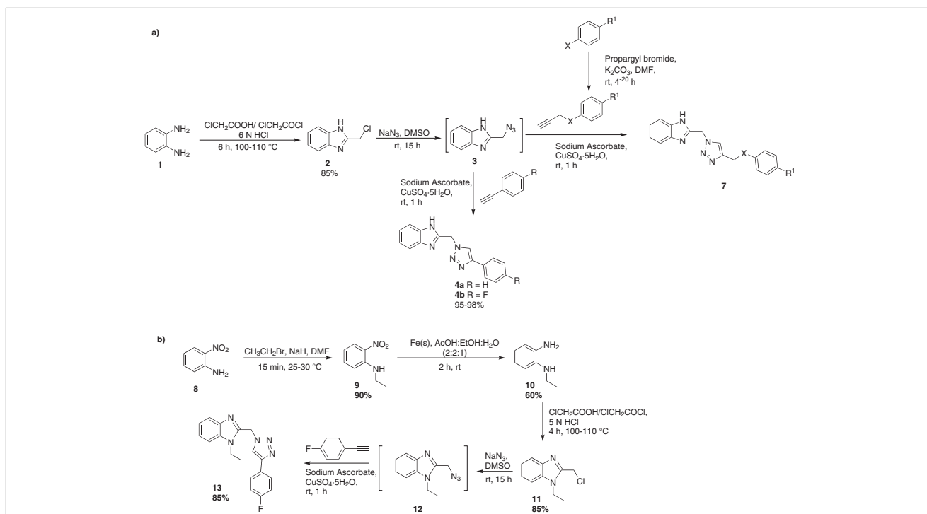
Scheme 12 (a) Synthesis of N -((1-((1 H -benzo[ d ]imidazol-2-yl)methyl)-1 H -1,2,3-triazol-4-yl)methyl)aniline and 2-((4-phenyl-1 H -1,2,3-triazol-1-yl)methyl)-1 H -benzo[ d ]imidazole derivatives; (b) synthesis of 1-ethyl-2-((4-(4-fluorophenyl)-1 H -1,2,3-triazol-1-yl)methyl)-1 H -benzo[ d ]imidazole 77
