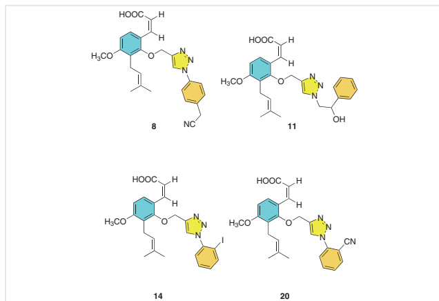
Figure 16 Structure of osthol-based triazole compounds 8 , 11 , 14 , and 20 82
