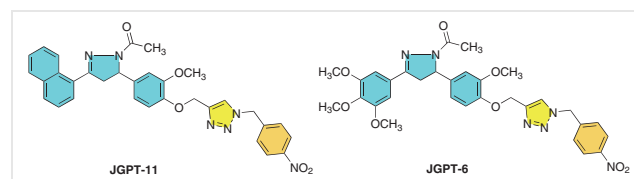
Figure 17 Structure of pyrazolyl-chalcone hybrids JGPT-6 and JGPT-11 84
