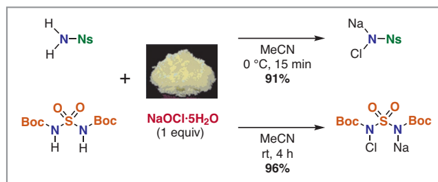
Scheme 3 Preparation of chloramine salts for anti - and syn -diamination reactions from simple amides with NaOCl pentahydrate
