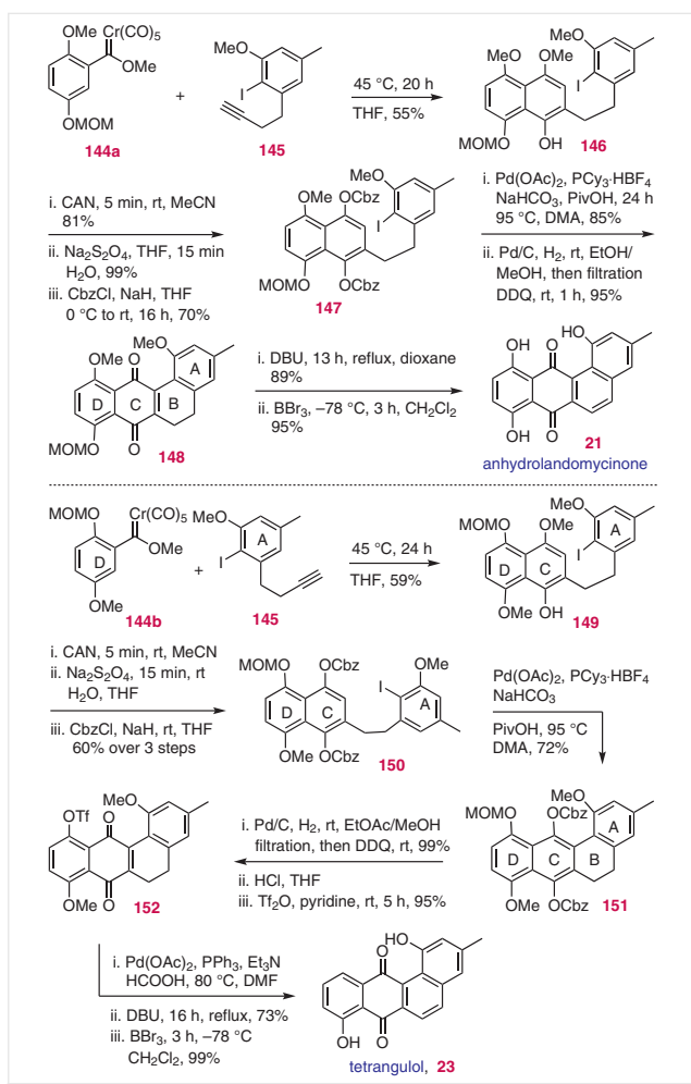
Scheme 26 Mong's total synthesis of anhydrolandomycinone ( 21 ) and tetrangulol ( 23 )
