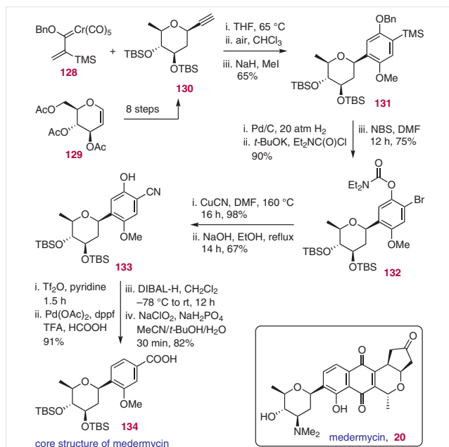
Scheme 24 Hong's synthesis of the medermycin core structure
