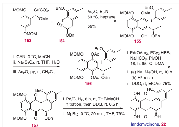
Scheme 27 Mong's total synthesis of landomycinone ( 22 )
