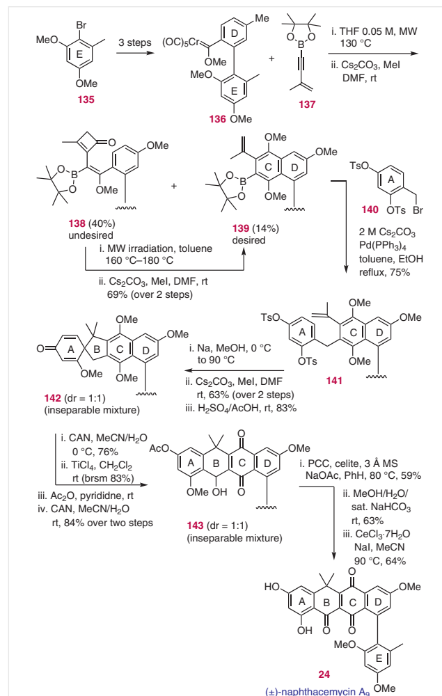
Scheme 25 Ōmura's synthesis of ( \pm )-naphthacemycin A 9 ( 24 )
