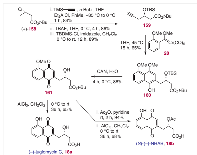
Scheme 28 Fernandes' syntheses of (–)-juglomycin C ( 18a ) and (–)-NHAB ( 18b )
