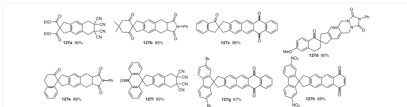
Figure 7 Compounds prepared by [2+2+2] cycloaddition followed by DA reaction
