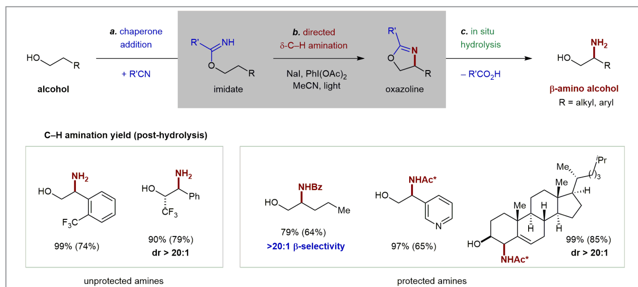
Scheme 1 Radical relay chaperone strategy for \beta -C–H amination of alcohols (Ac* = COCl 2 )
