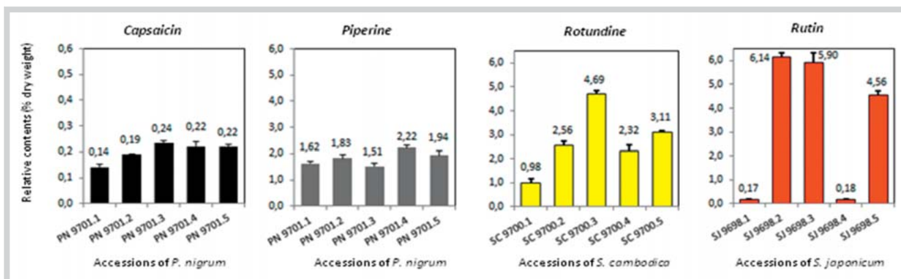
Fig. 1 HPLC quantification of extract compounds. Quantification of capsaicin and piperine in fruits of P. nigrum , of rotundine in mixture of tubers and roots of S. cambodica and of rutin in flower buds of S. japonicum .
