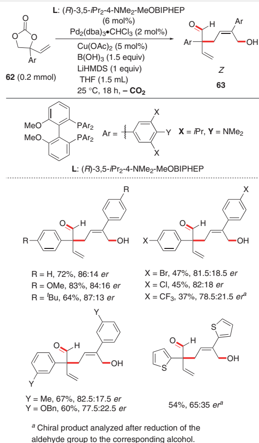
Scheme 14 Substrate scope for the synthesis of targets 63
