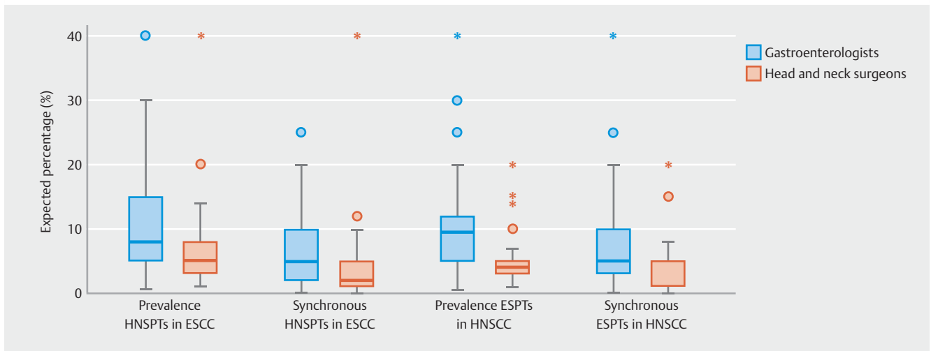
► Fig. 1 The expected prevalence of HNSPTs in patients with ESCC and vice versa in a Western population. ESCC, esophageal squamous cell carcinoma; ESPT, esophageal second primary tumor; HNSPT, head and neck second primary tumor; HNSCC, head and neck squamous cell carcinoma; HNSPT, head and neck second primary tumors. Boxplot legend: median (midline), box (25th to 75th percentiles) and whiskers. Outliers and extreme values beyond the whiskers are shown with circles and asterisks, respectively. Outliers with an expected prevalence of above 40% not shown (n=5)
