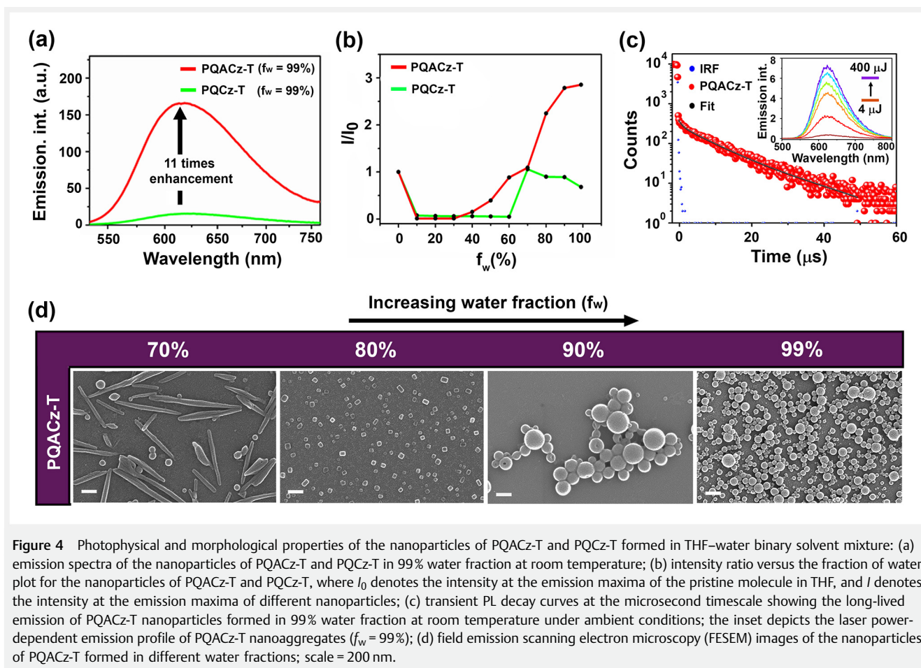
Figure 4 Photophysical and morphological properties of the nanoparticles of PQACz-T and PQCz-T formed in THF–water binary solvent mixture: (a) emission spectra of the nanoparticles of PQACz-T and PQCz-T in 99% water fraction at room temperature; (b) intensity ratio versus the fraction of water plot for the nanoparticles of PQACz-T and PQCz-T, where I_0 denotes the intensity at the emission maxima of the pristine molecule in THF, and I denotes the intensity at the emission maxima of different nanoparticles; (c) transient PL decay curves at the microsecond timescale showing the long-lived emission of PQACz-T nanoparticles formed in 99% water fraction at room temperature under ambient conditions; the inset depicts the laser power-dependent emission profile of PQACz-T nanoaggregates ( f_w = 99\% ); (d) field emission scanning electron microscopy (FESEM) images of the nanoparticles of PQACz-T formed in different water fractions; scale = 200 nm.
