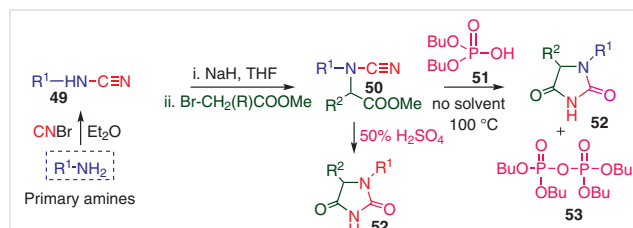
Scheme 4 Novel route for the synthesis of hydantoins
