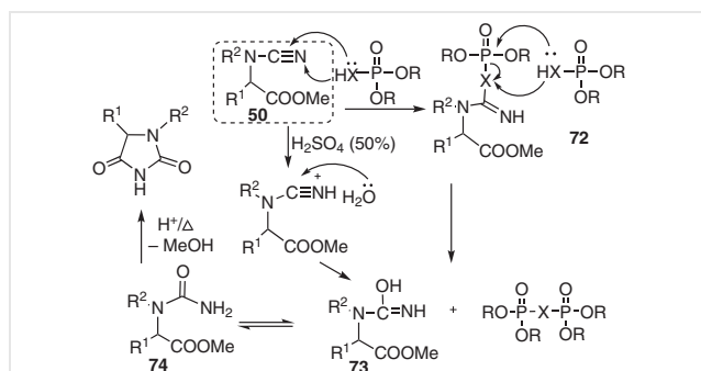
Scheme 5 Mechanism for the formation of hydantoin from methyl (cyanoamino)acetates 50
