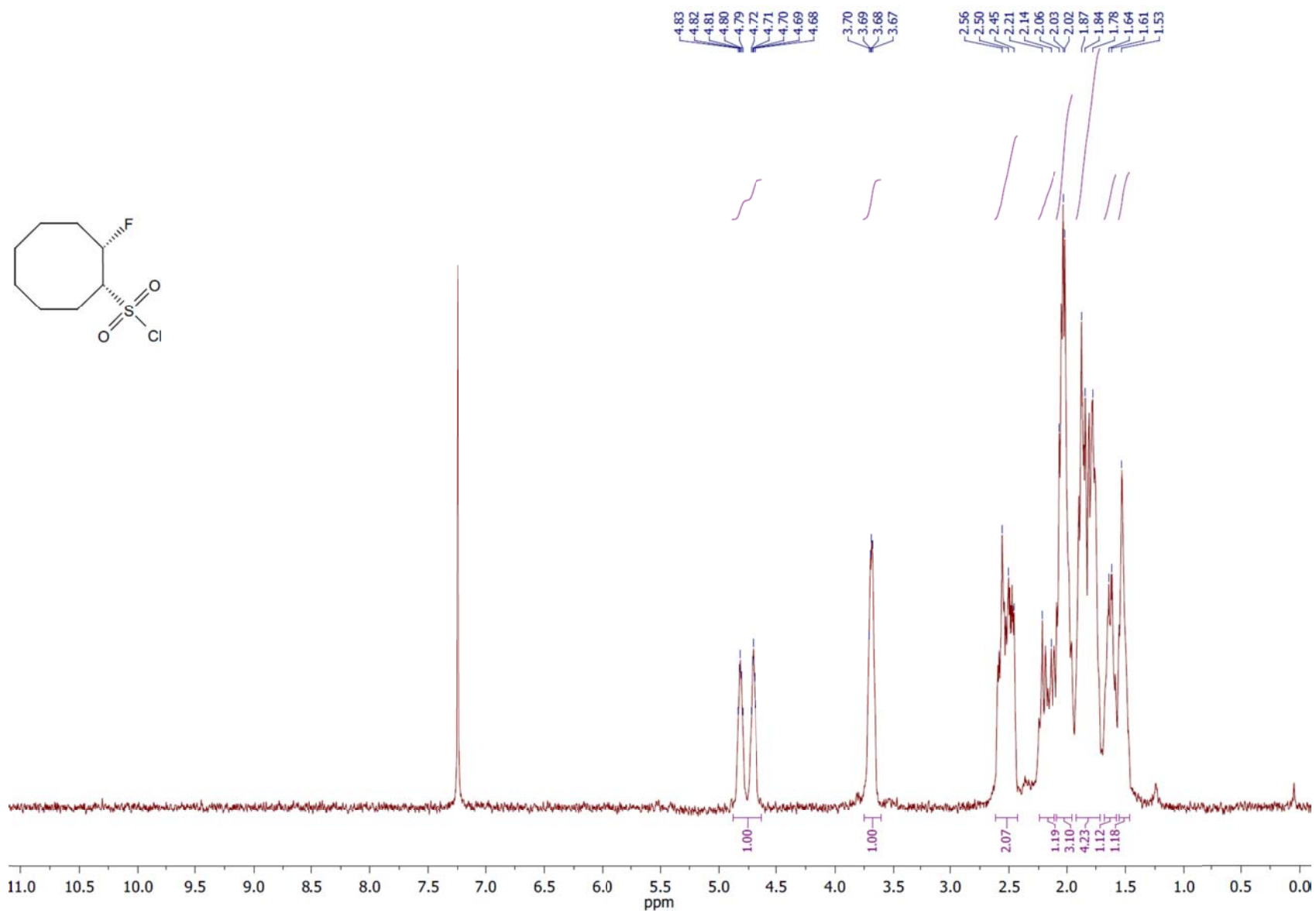
1 H NMR spectrum of the compound 4u .
