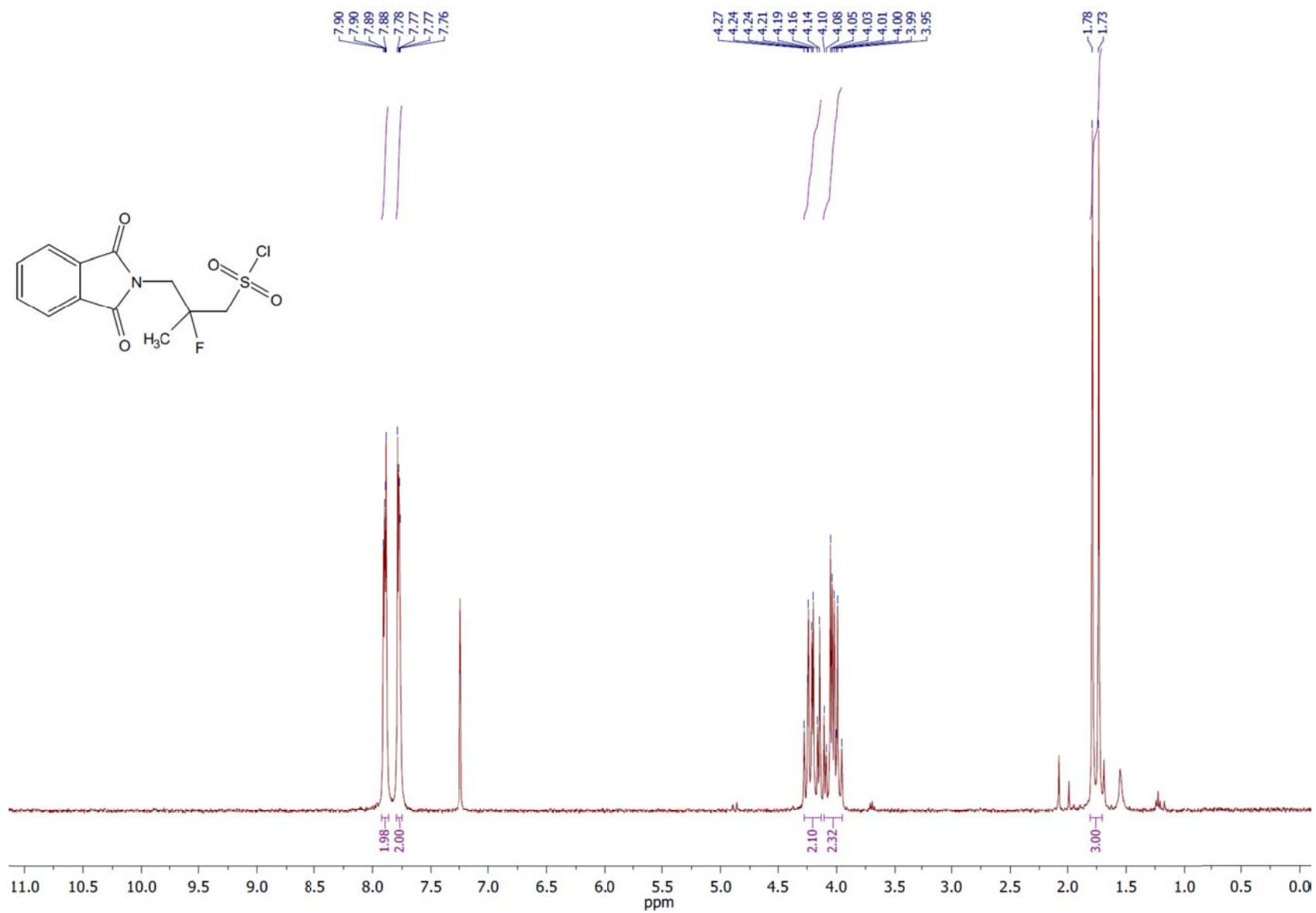
1 H NMR spectrum of the compound 4d .
