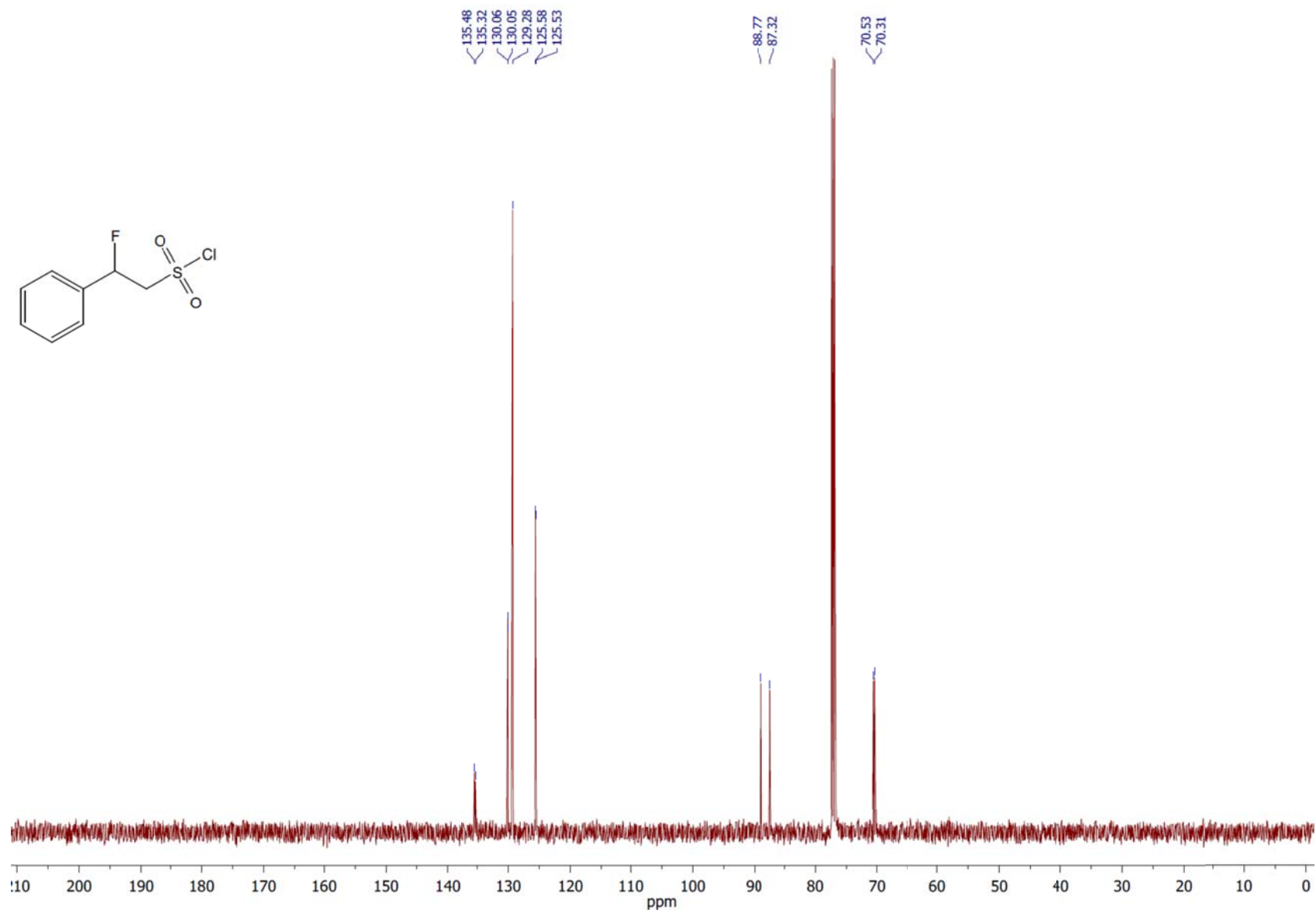
^{13}\text{C} NMR spectrum of the compound 4a .
