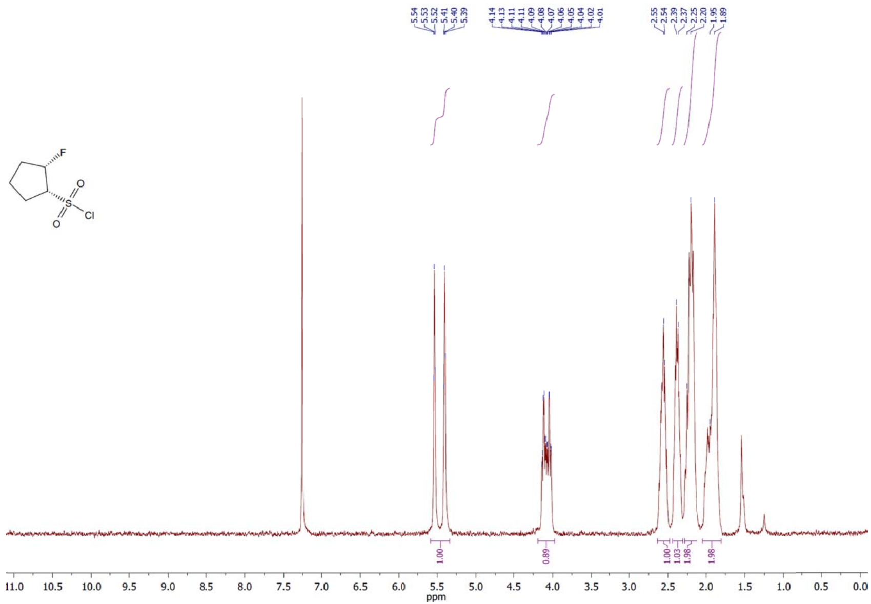
1 H NMR spectrum of the compound 4r .
