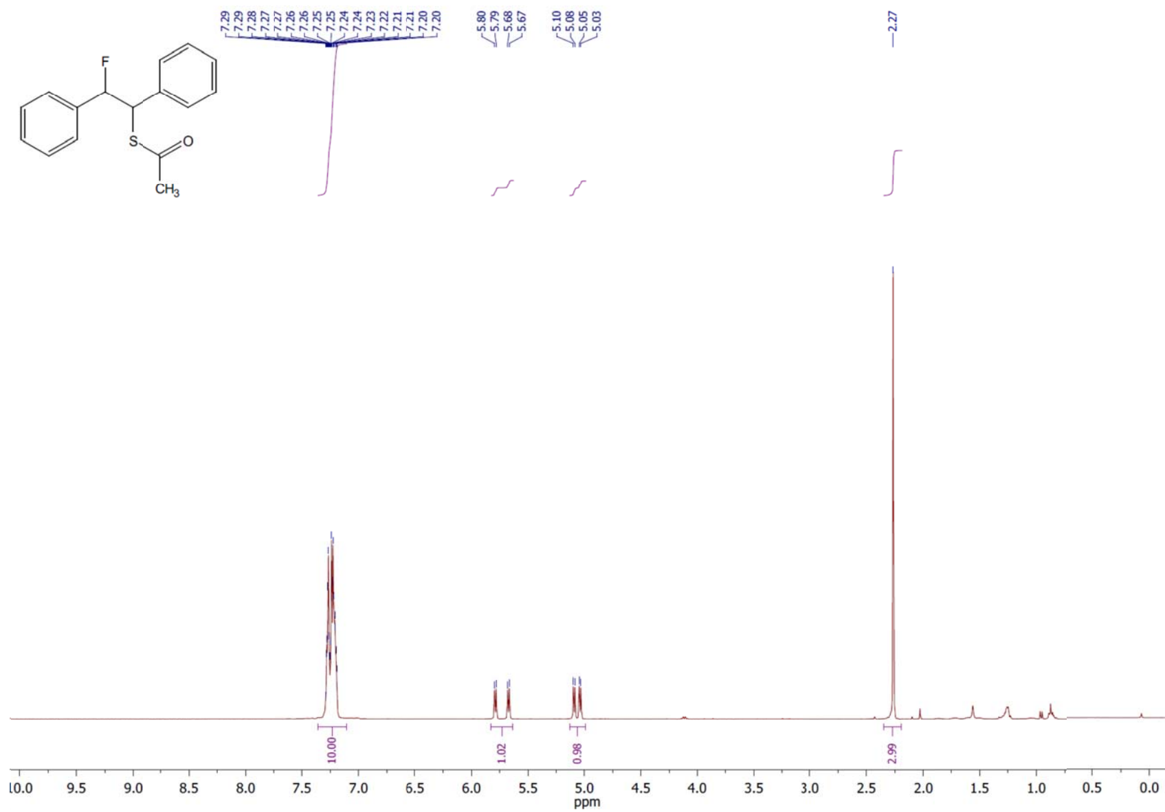
1 H NMR spectrum of the compound 3f .
