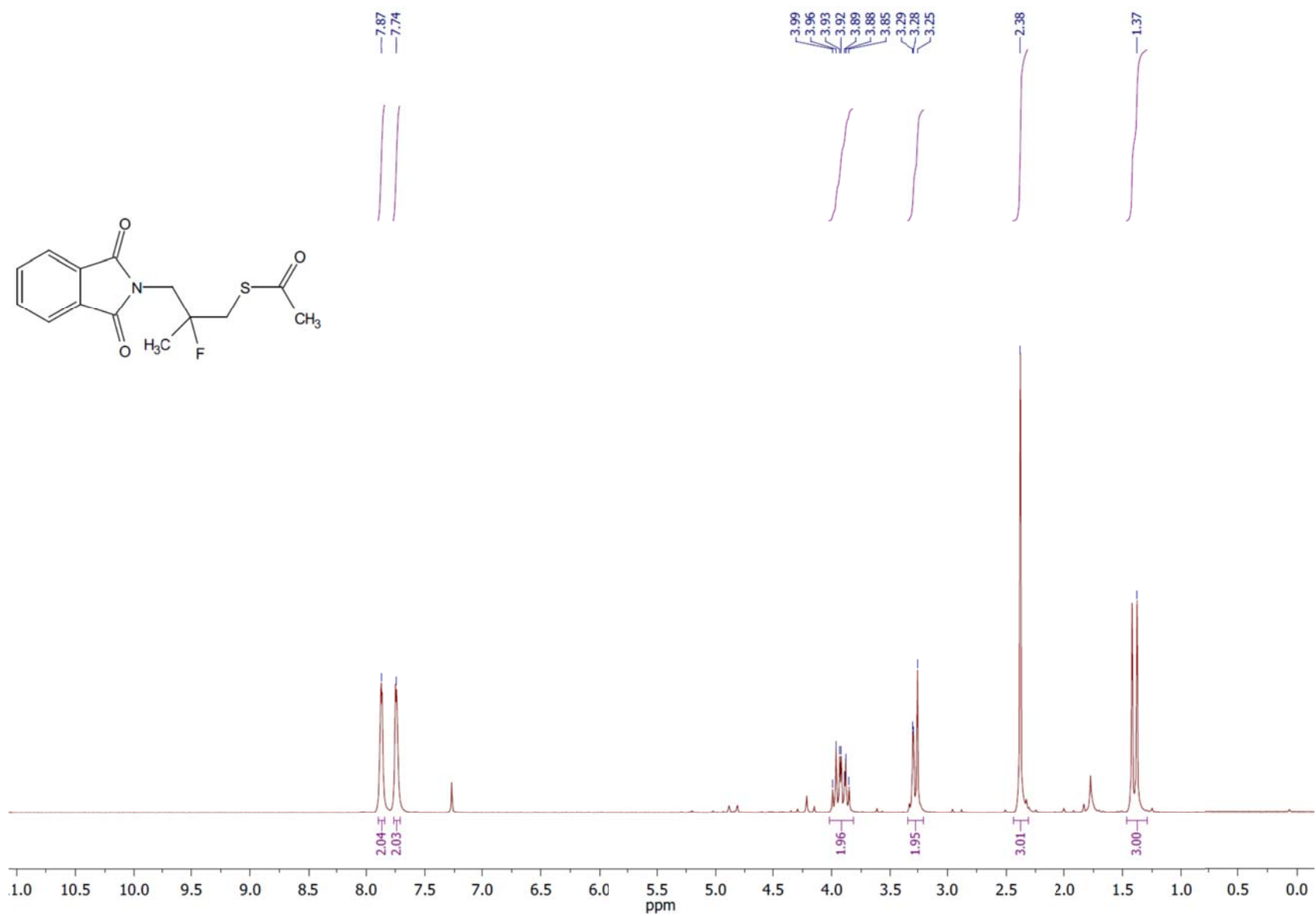
1 H NMR spectrum of the compound 3d .
