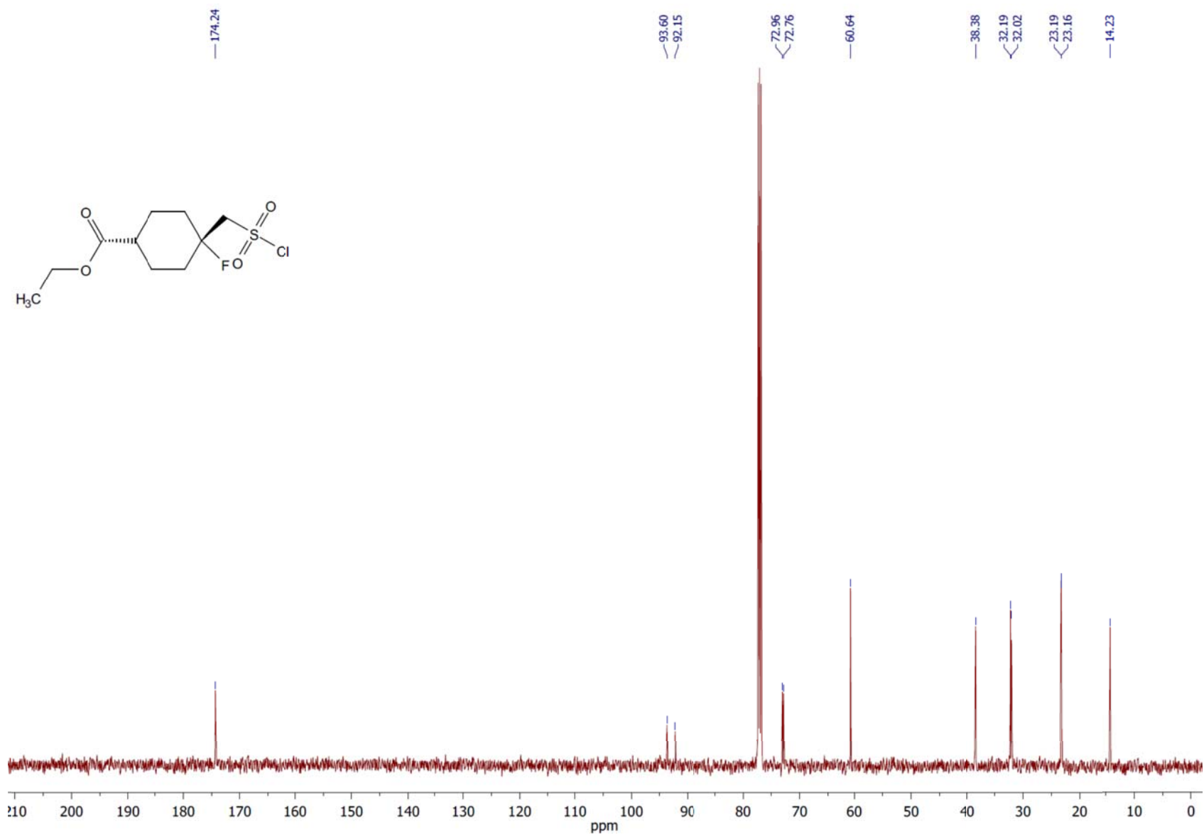
13 C NMR spectrum of the compound 4m .
