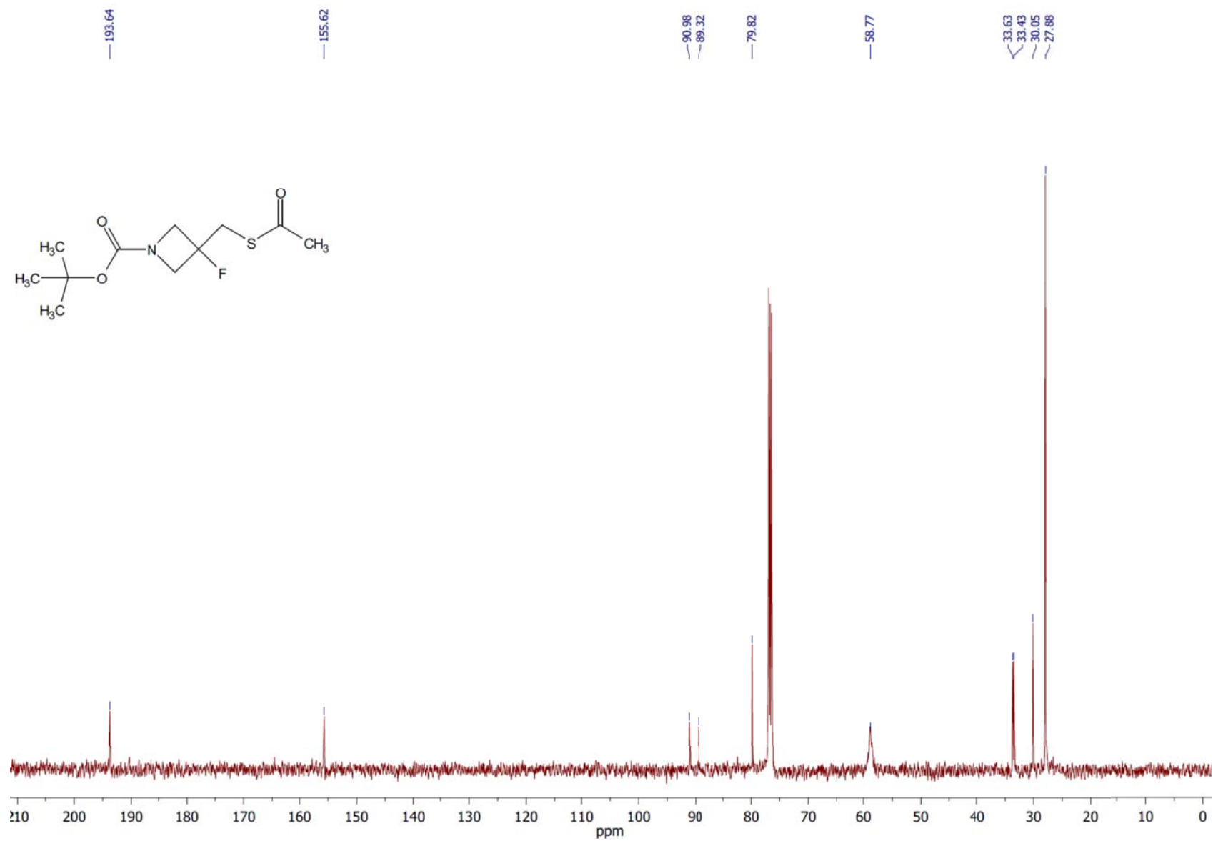
^{13}\text{C} NMR spectrum of the compound 3n .
