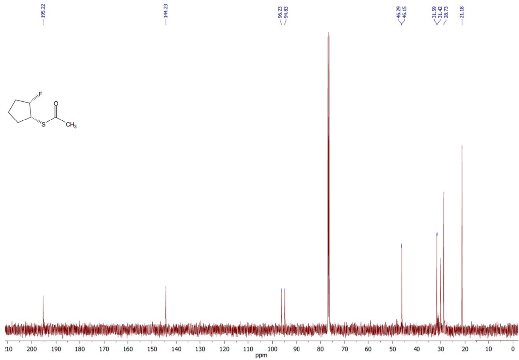
^{13}\text{C} NMR spectrum of the compound 3r .
