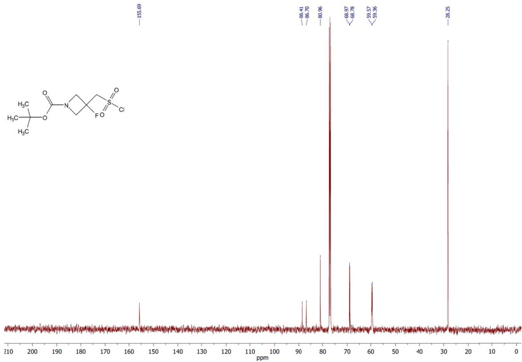
^{13}\text{C} NMR spectrum of the compound 4n .
