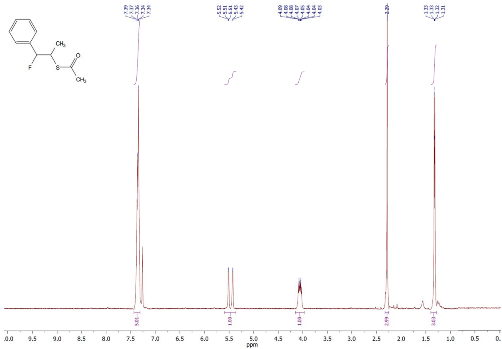
1 H NMR spectrum of the compound 3e .
