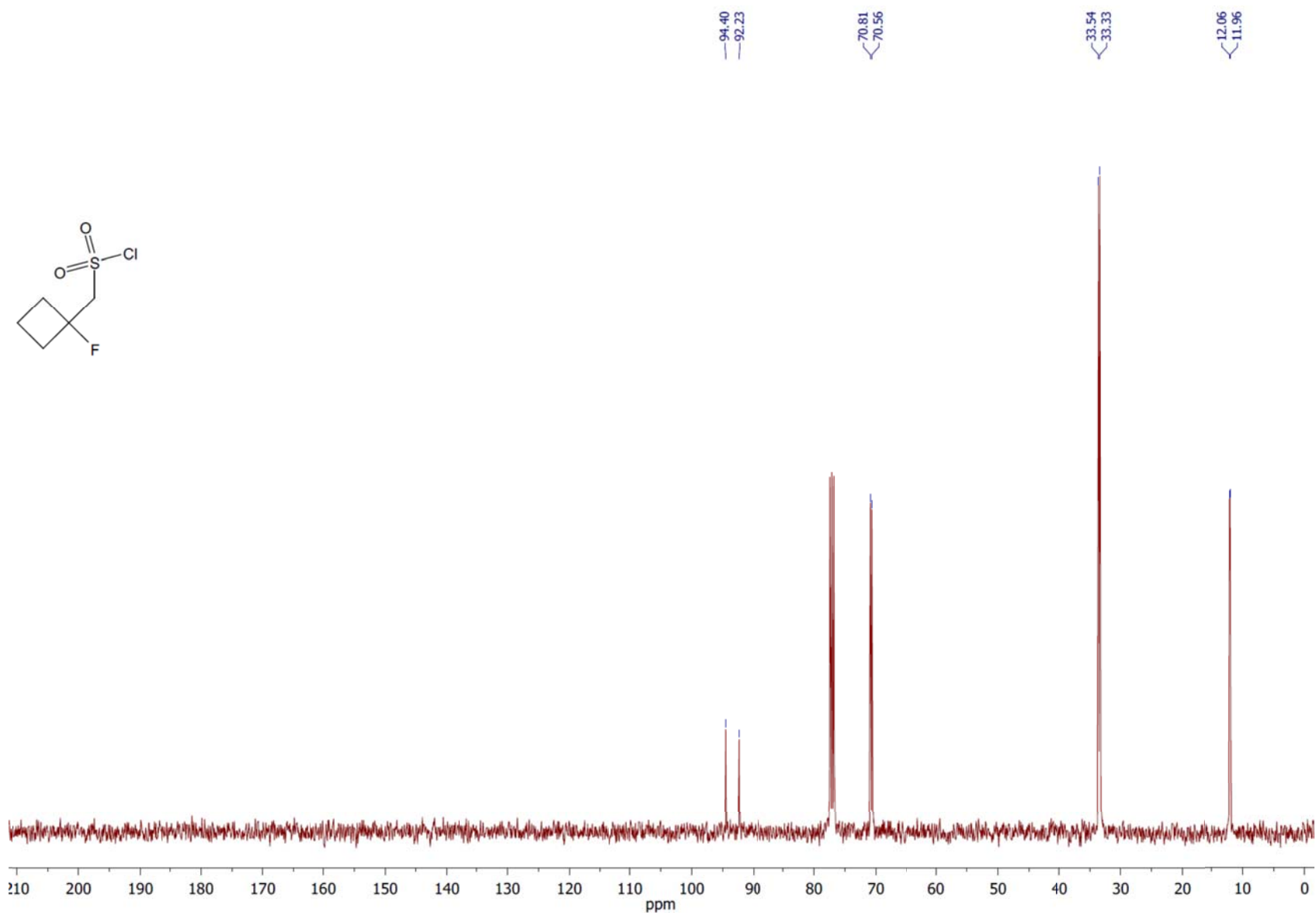
^{13}\text{C} NMR spectrum of the compound 4h .
