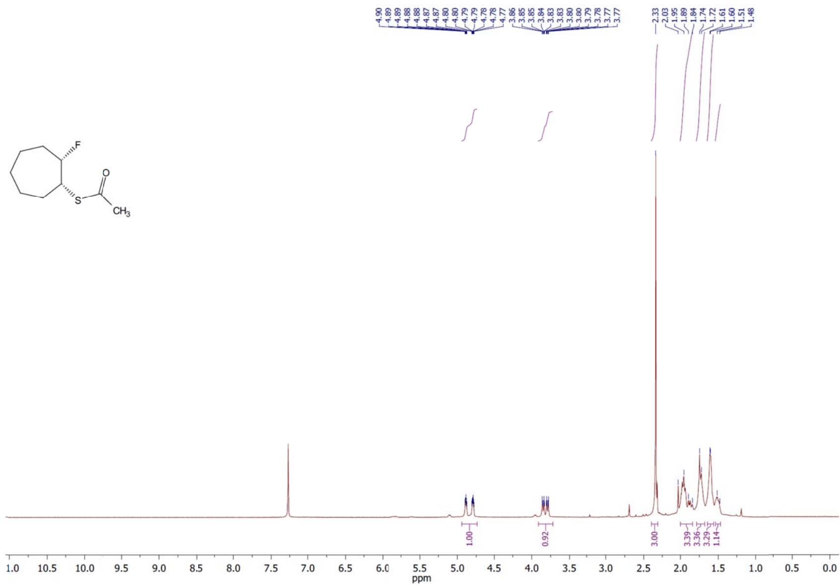
^1\text{H} NMR spectrum of the compound 3t .
