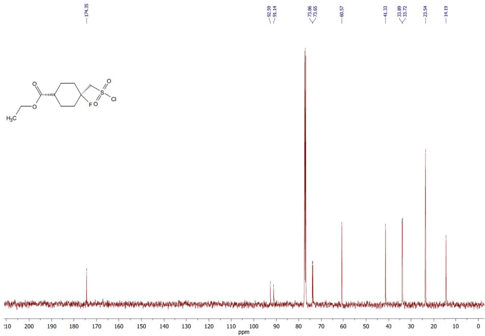
^{13}\text{C} NMR spectrum of the compound 41 .
