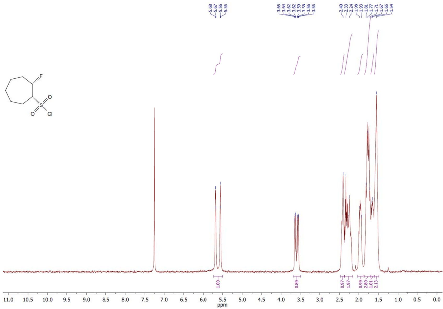
1 H NMR spectrum of the compound 4t .
