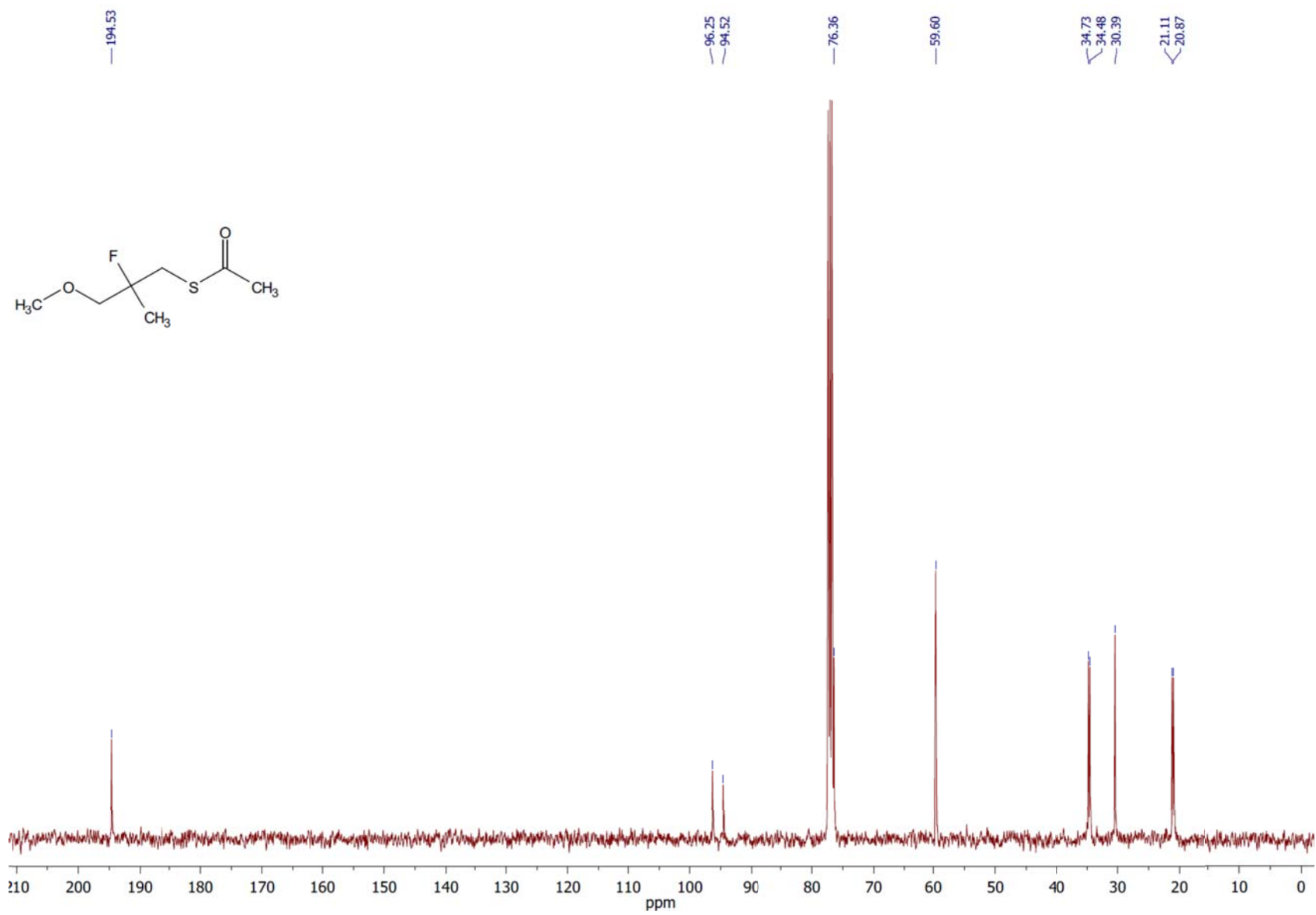
^{13}\text{C} NMR spectrum of the compound 3b .
