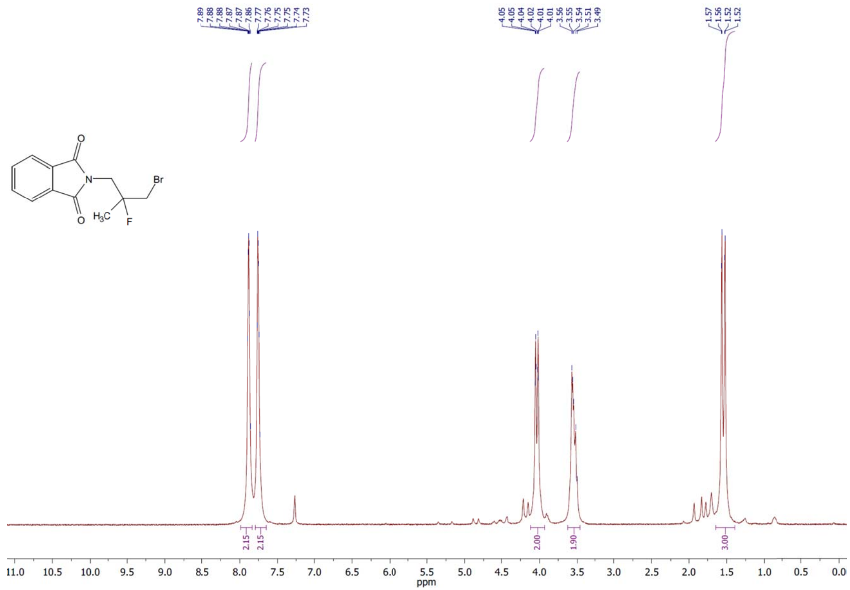
1 H NMR spectrum of the compound 2d .
