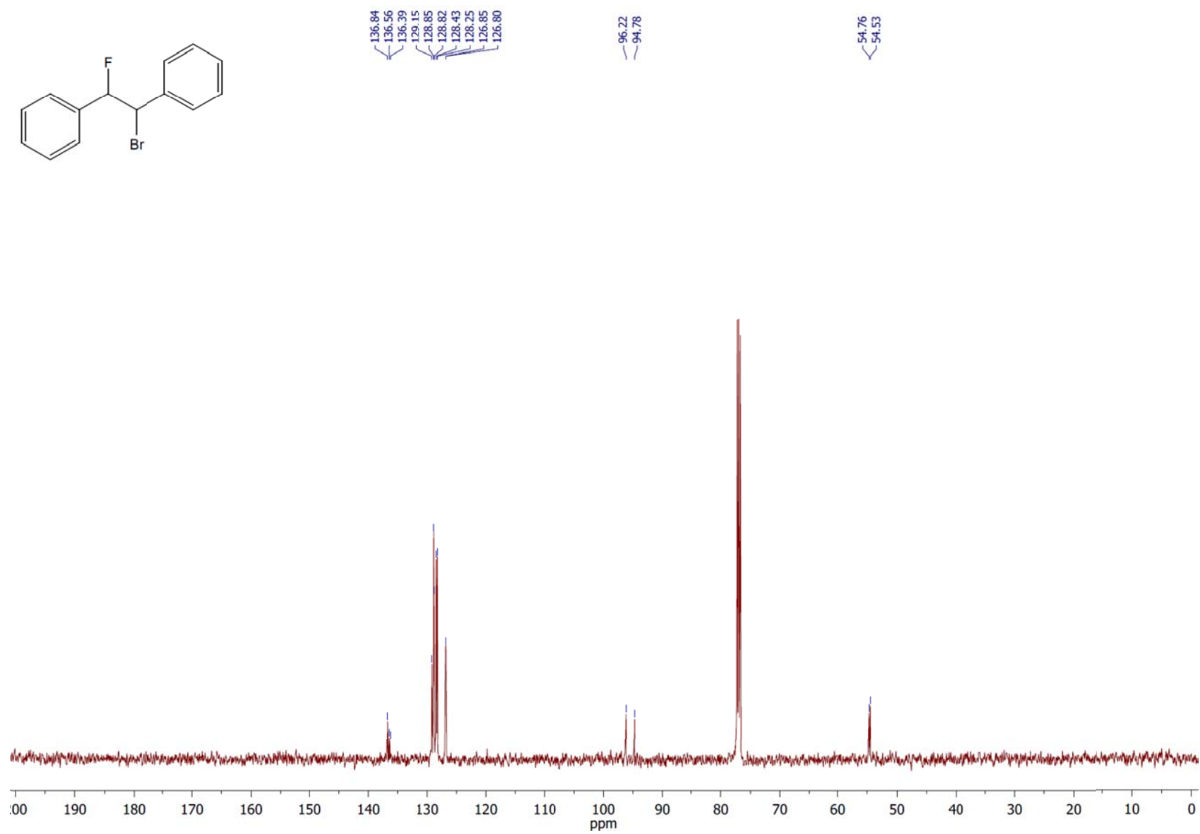
^{13}\text{C} NMR spectrum of the compound 2f .
