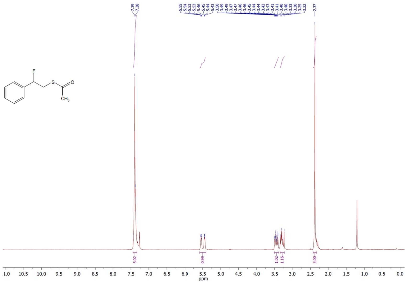
1 H NMR spectrum of the compound 3a .
