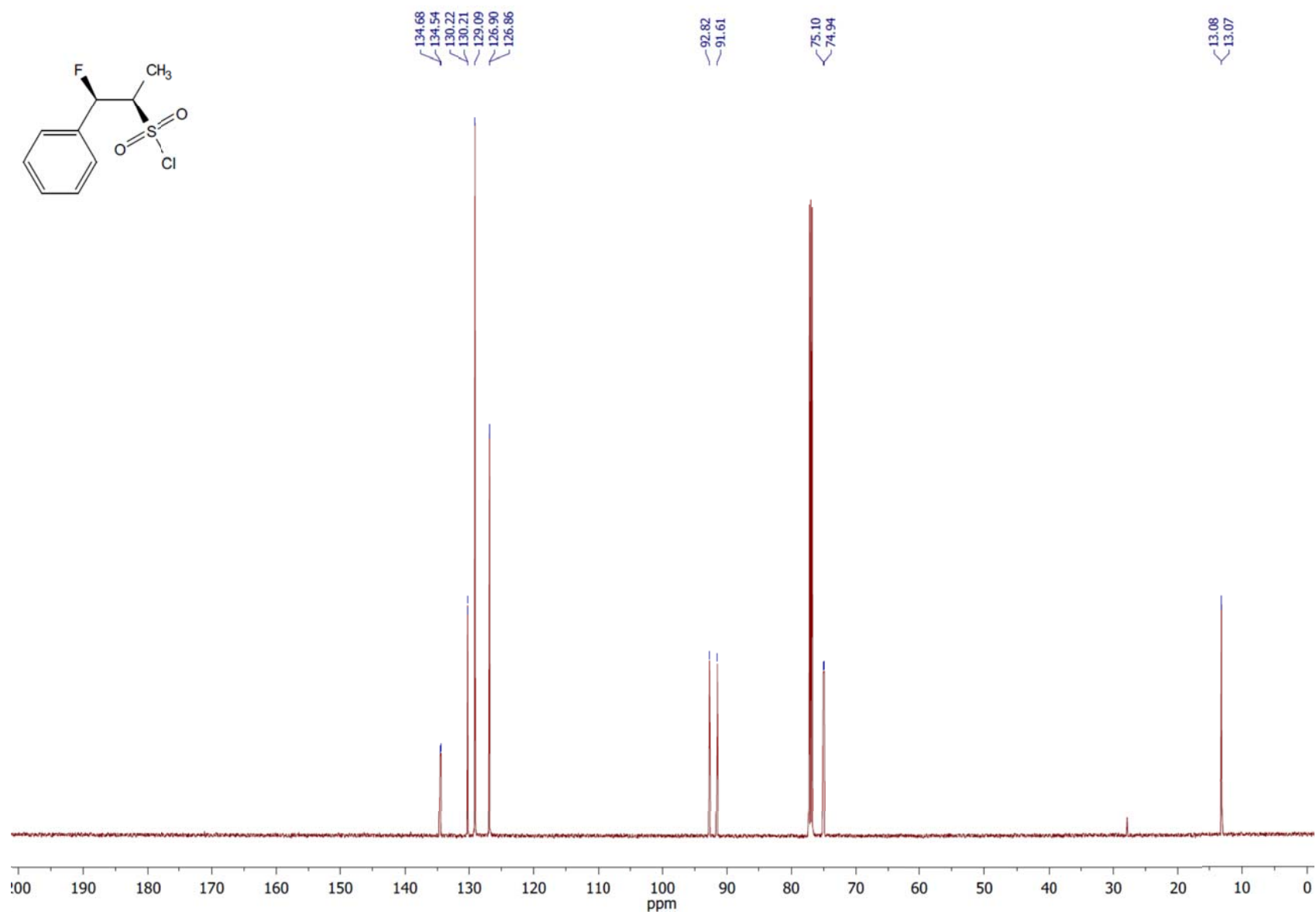
^{13}\text{C} NMR spectrum of the compound 4e .
