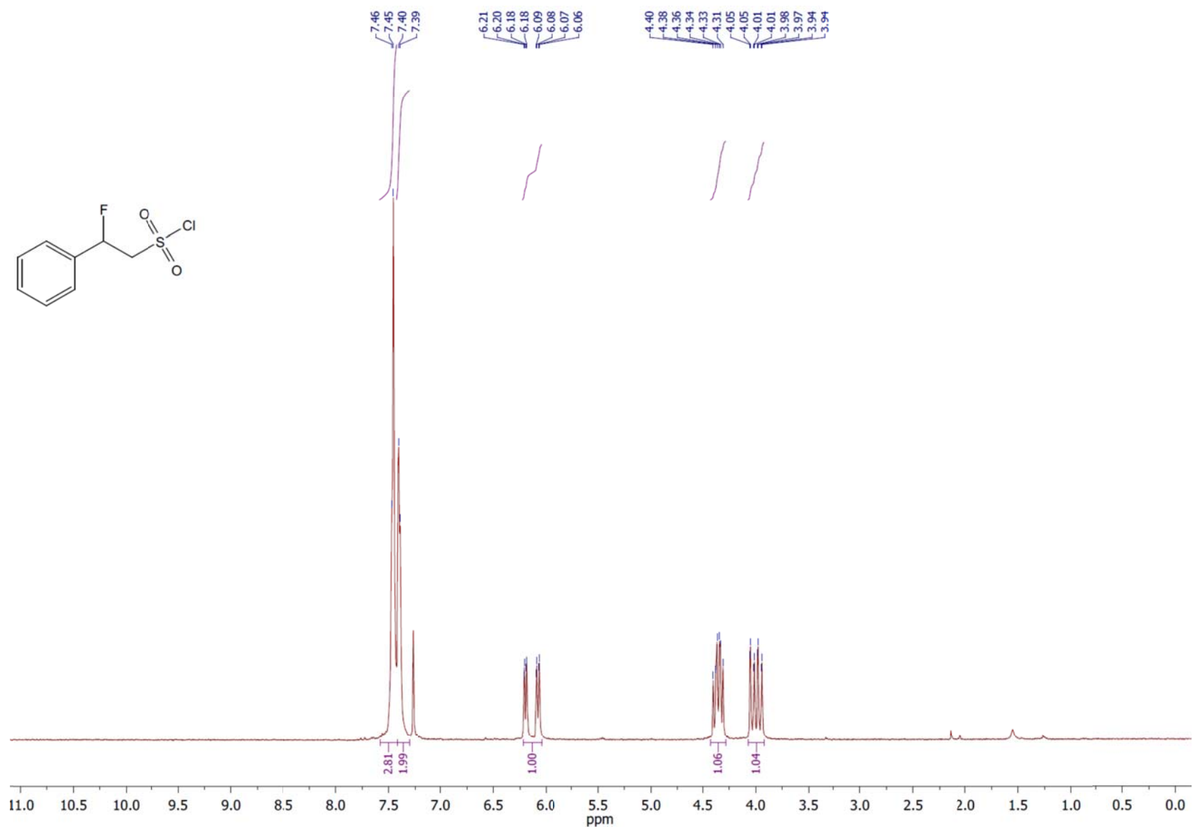
1 H NMR spectrum of the compound 4a .
