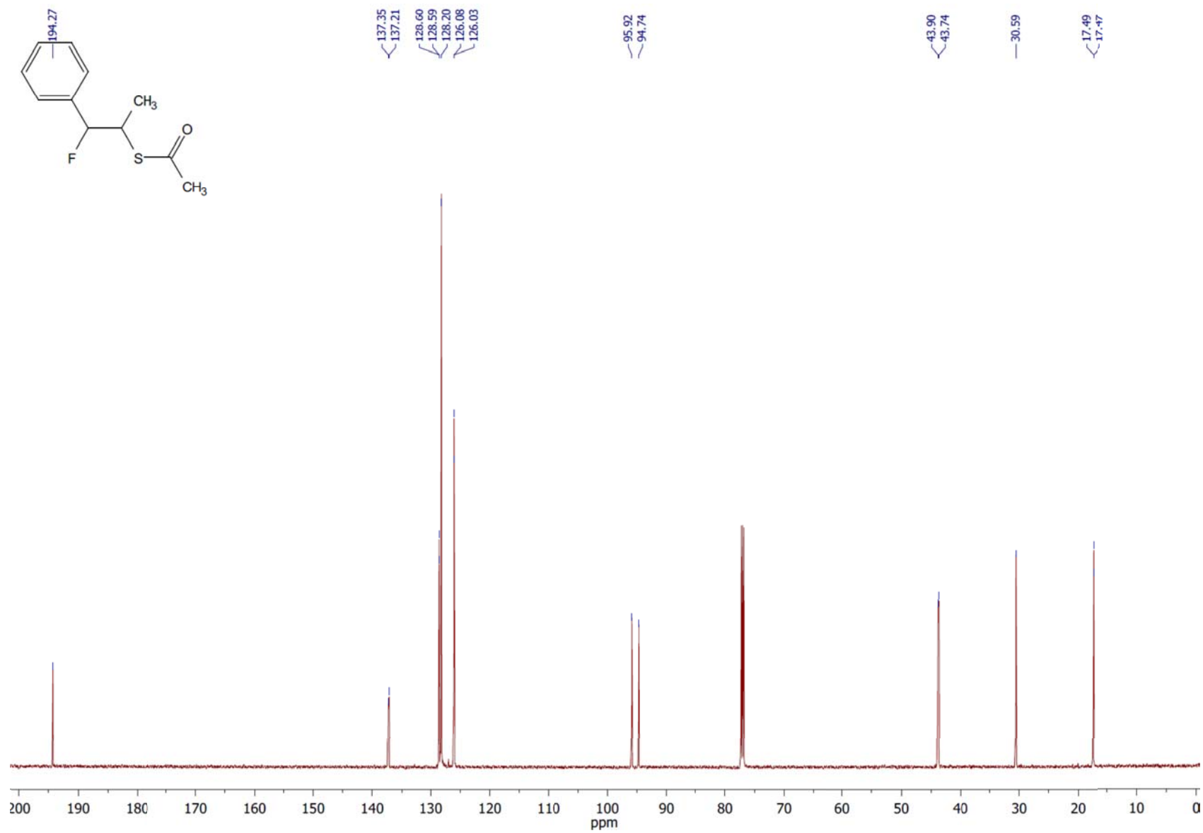
^{13}\text{C} NMR spectrum of the compound 3e .
