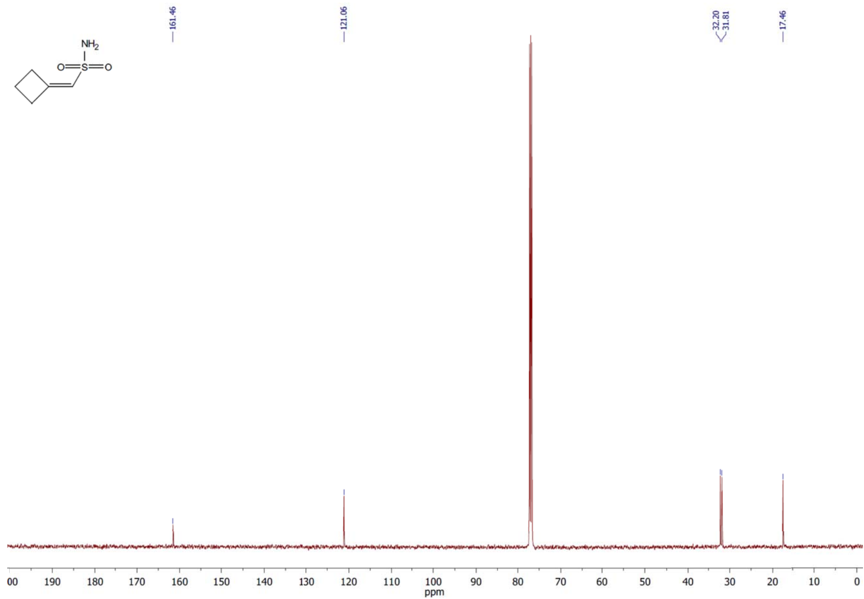
^{13}\text{C} NMR spectrum of the compound 8a .
