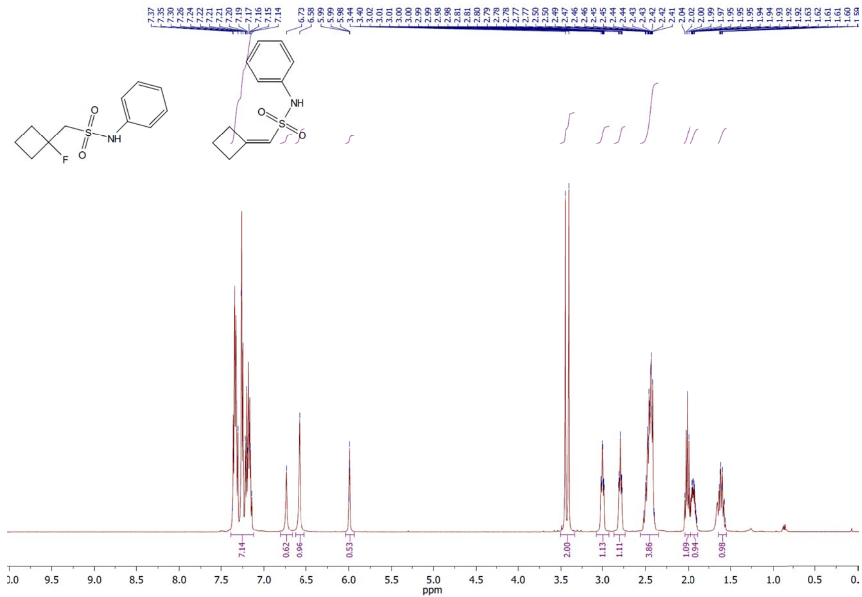
^1\text{H} NMR spectrum of a mixture of 7b and 8b (1.7:1).
