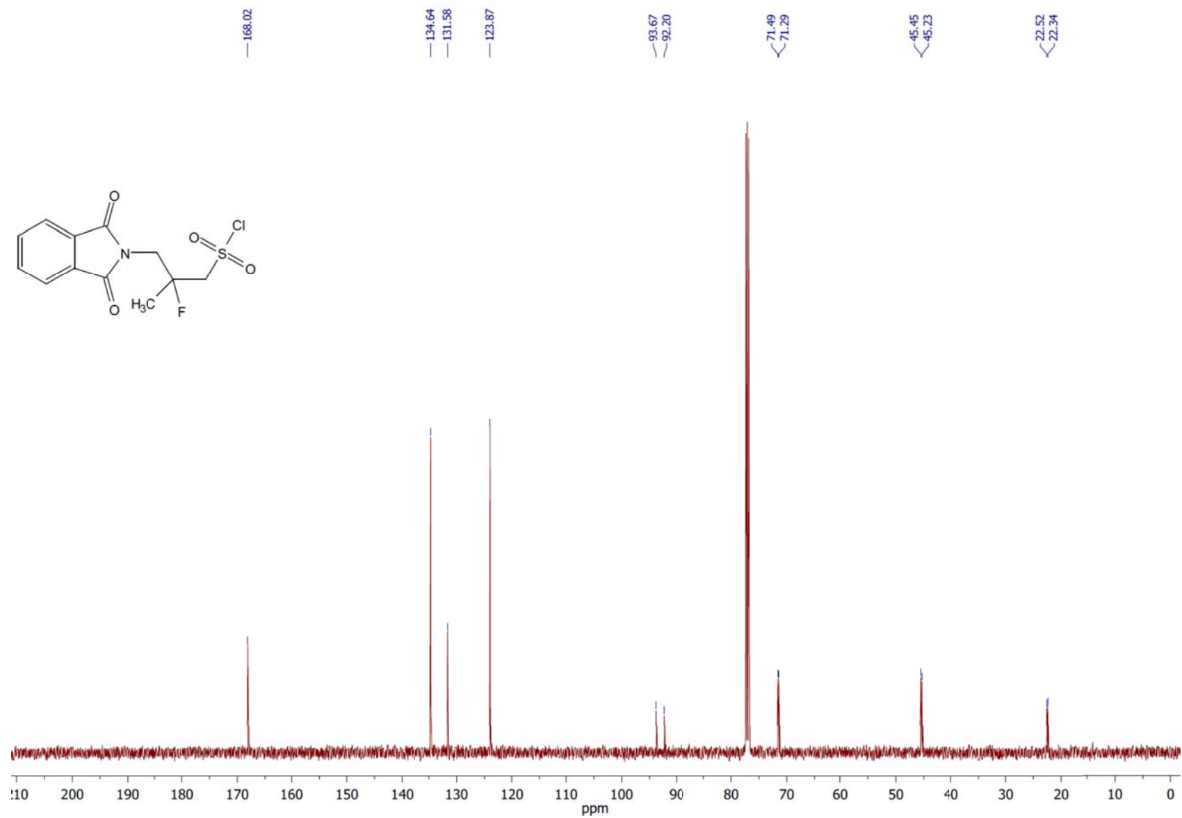
^{13}\text{C} NMR spectrum of the compound 4d .
