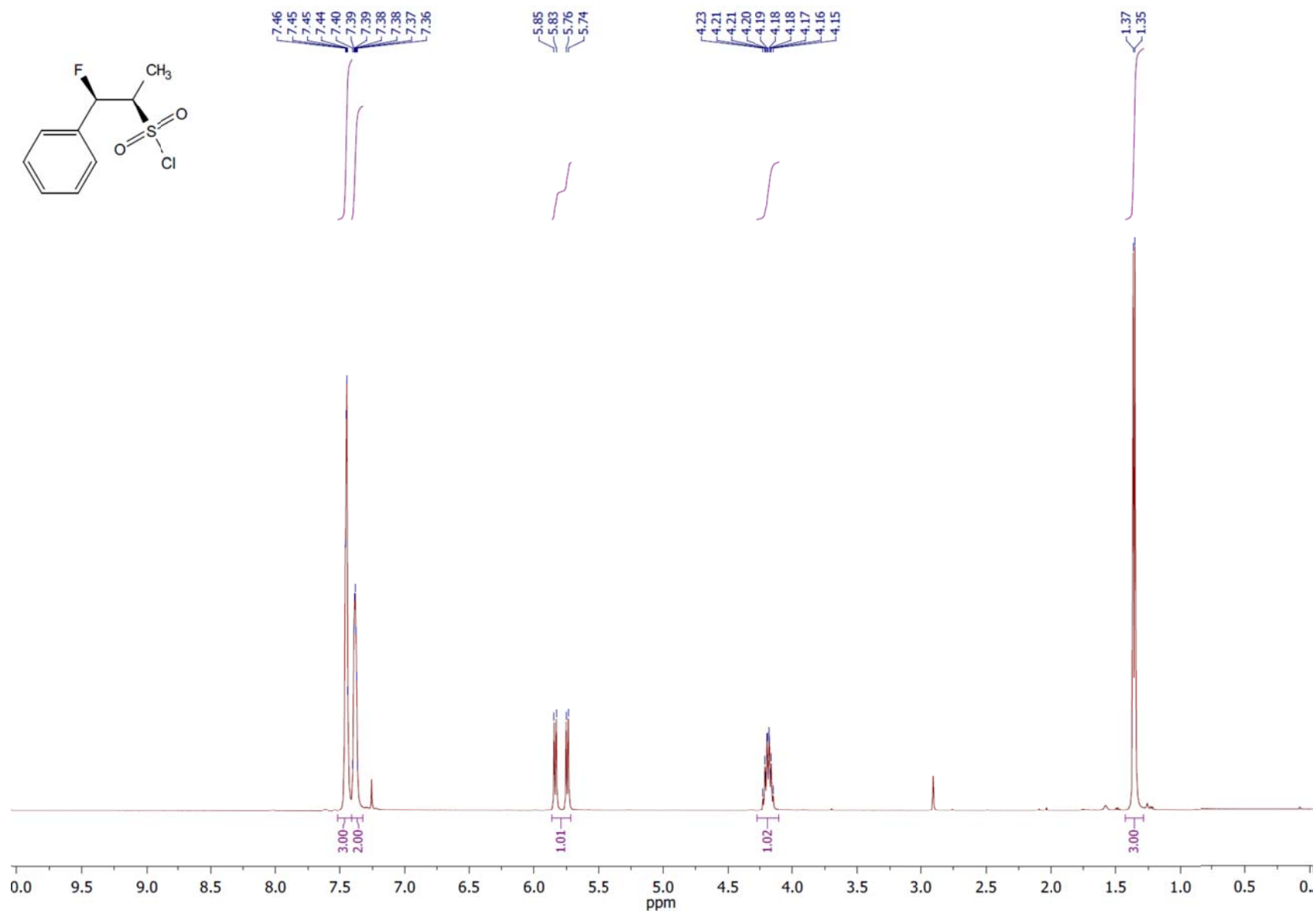
1 H NMR spectrum of the compound 4e .
