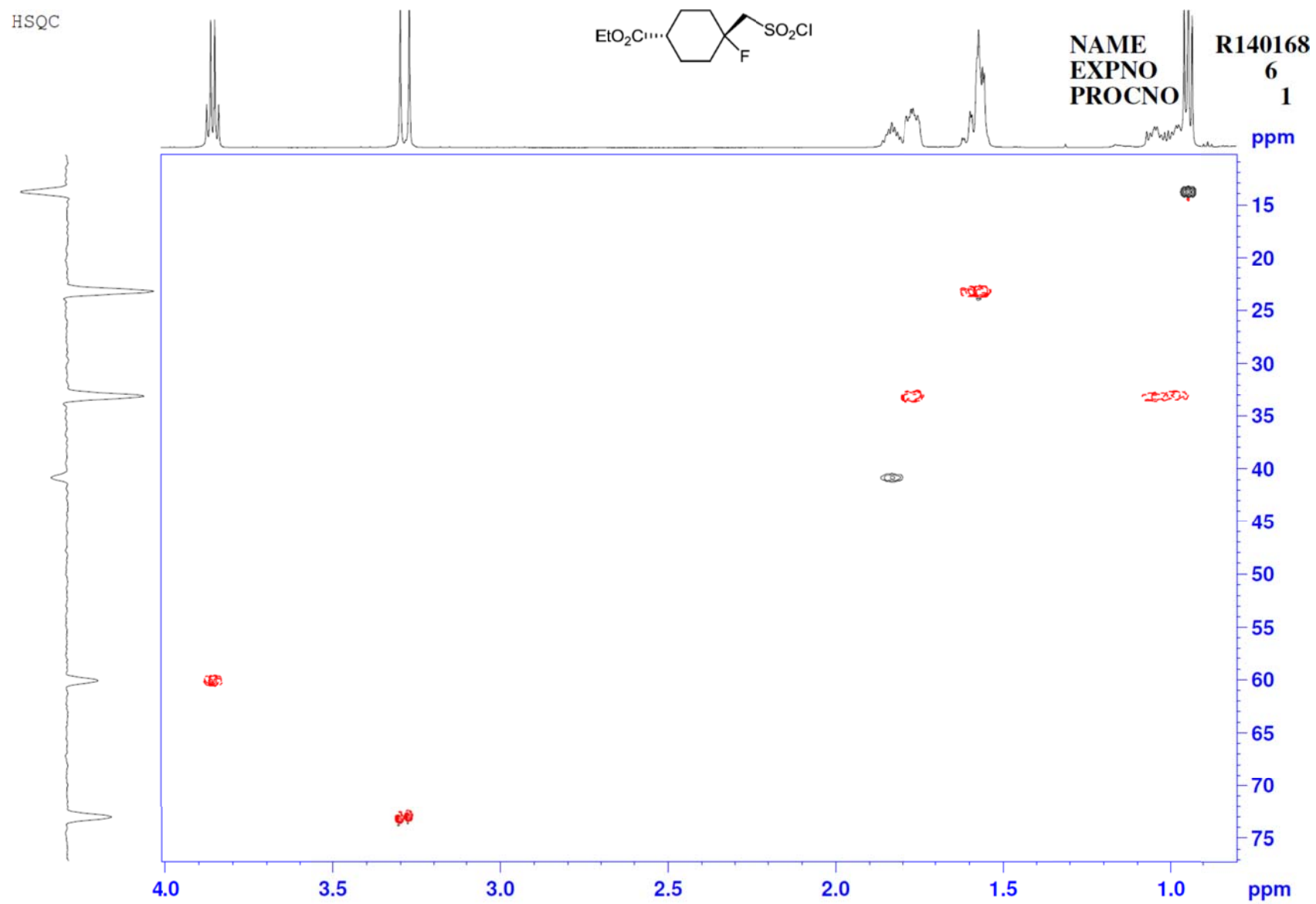
HSQC spectrum of the compound 4m .
