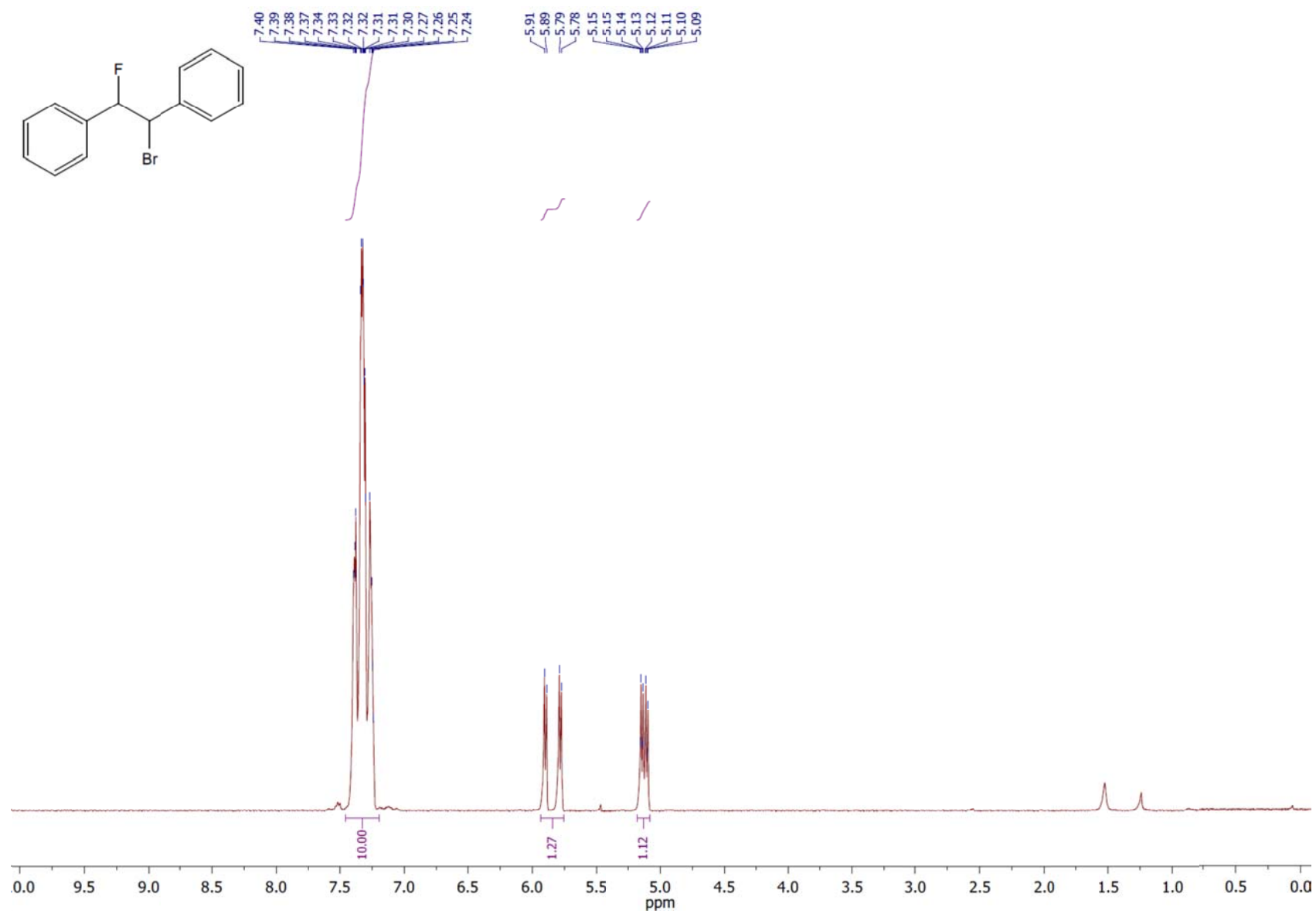
1 H NMR spectrum of the compound 2f .
