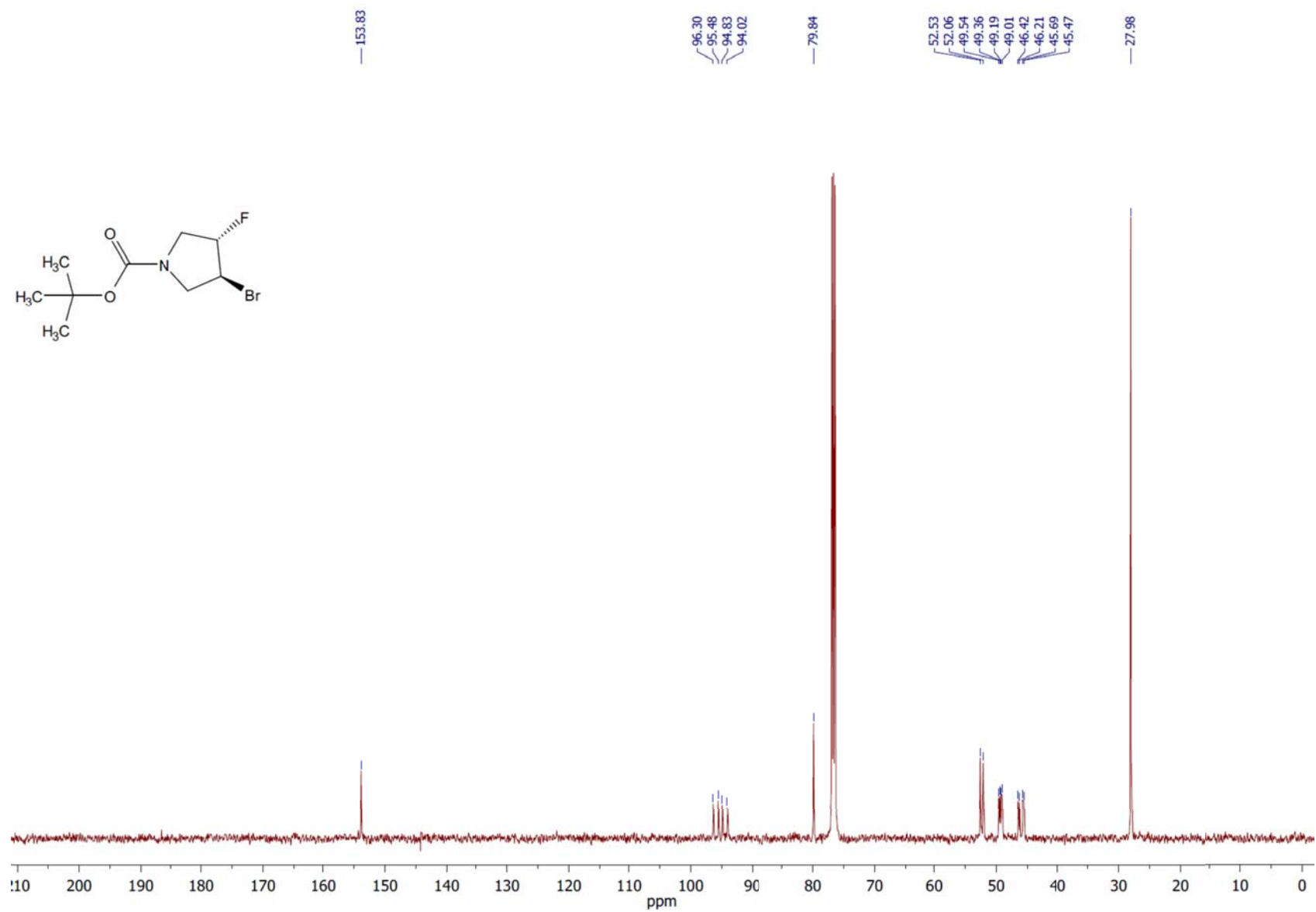
^{13}\text{C} NMR spectrum of the compound 2v .
