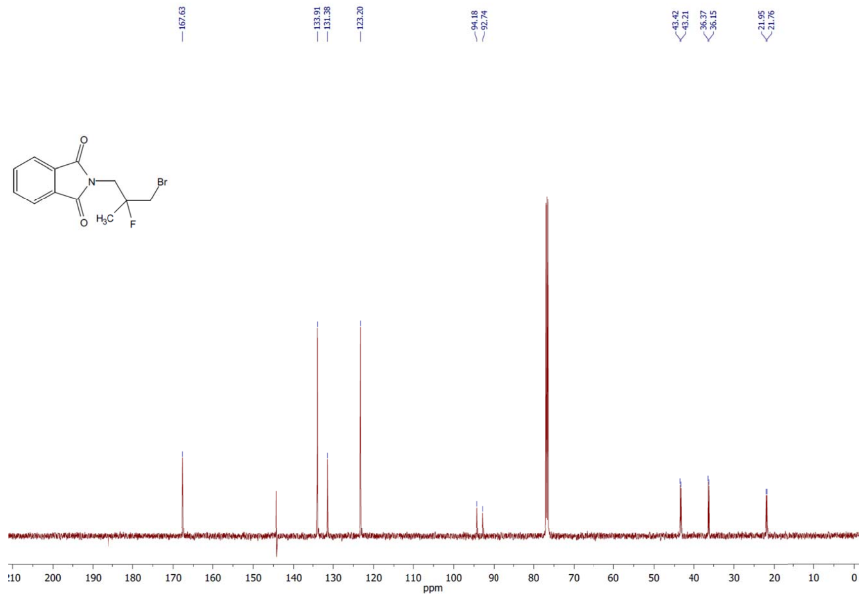
^{13}\text{C} NMR spectrum of the compound 2d .
