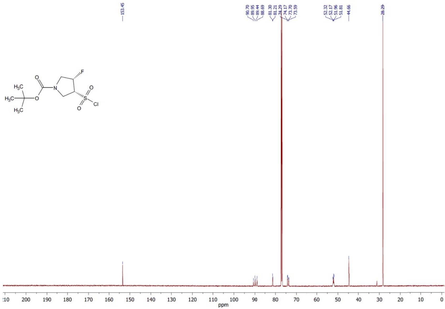
^{13}\text{C} NMR spectrum of the compound 4v .
