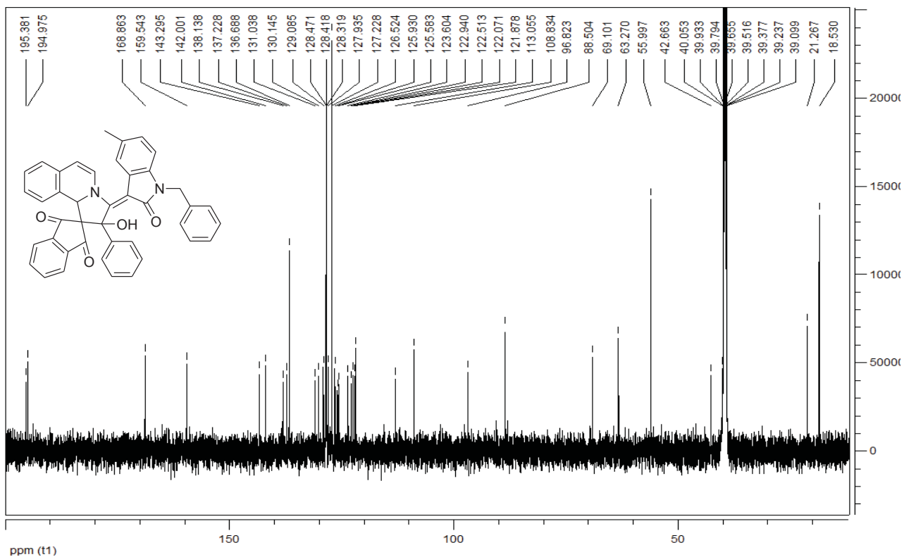
2'-Isatylidene spiro[indan-2,1'-pyrrolo[2,1-a]isoquinoline] 3k
