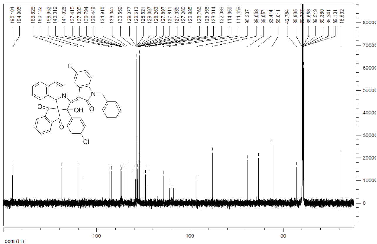
2'-Isatylidene spiro[indan-2,1'-pyrrolo[2,1-a]isoquinoline] 3n
