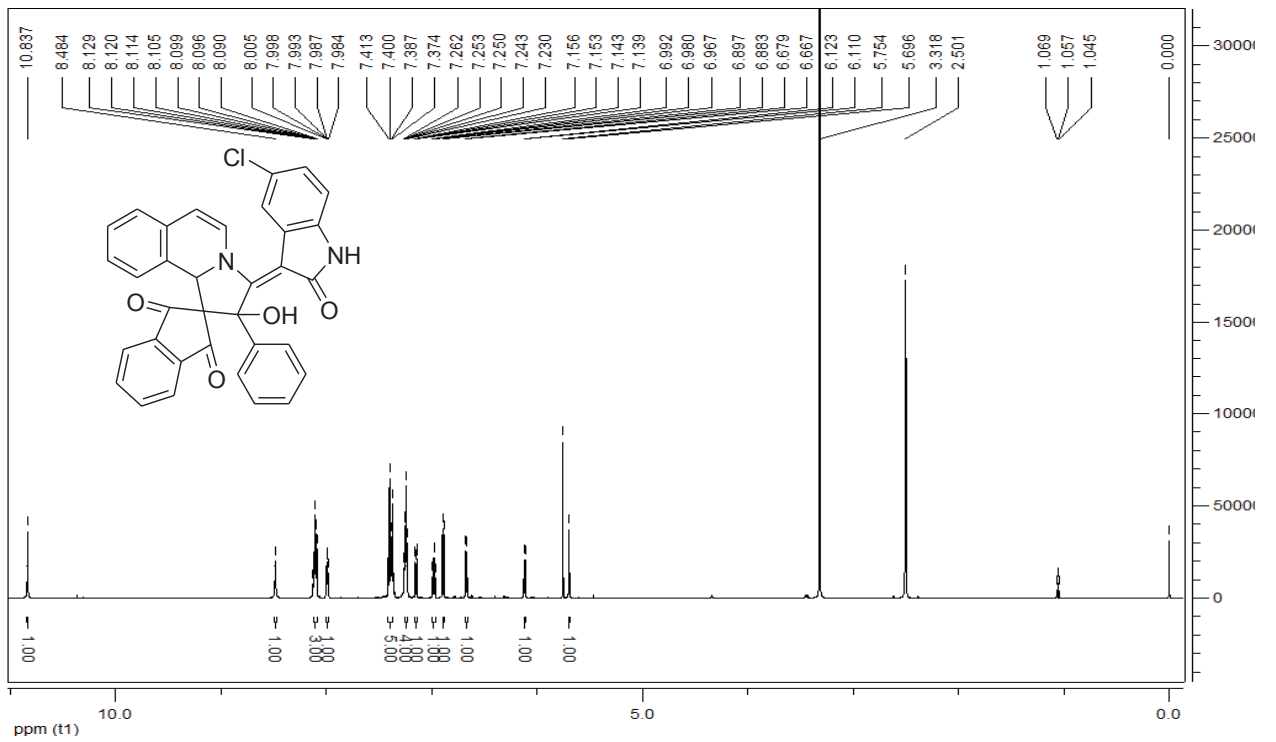
2'-Isatylidene spiro[indan-2,1'-pyrrolo[2,1-a]isoquinoline] 3d
