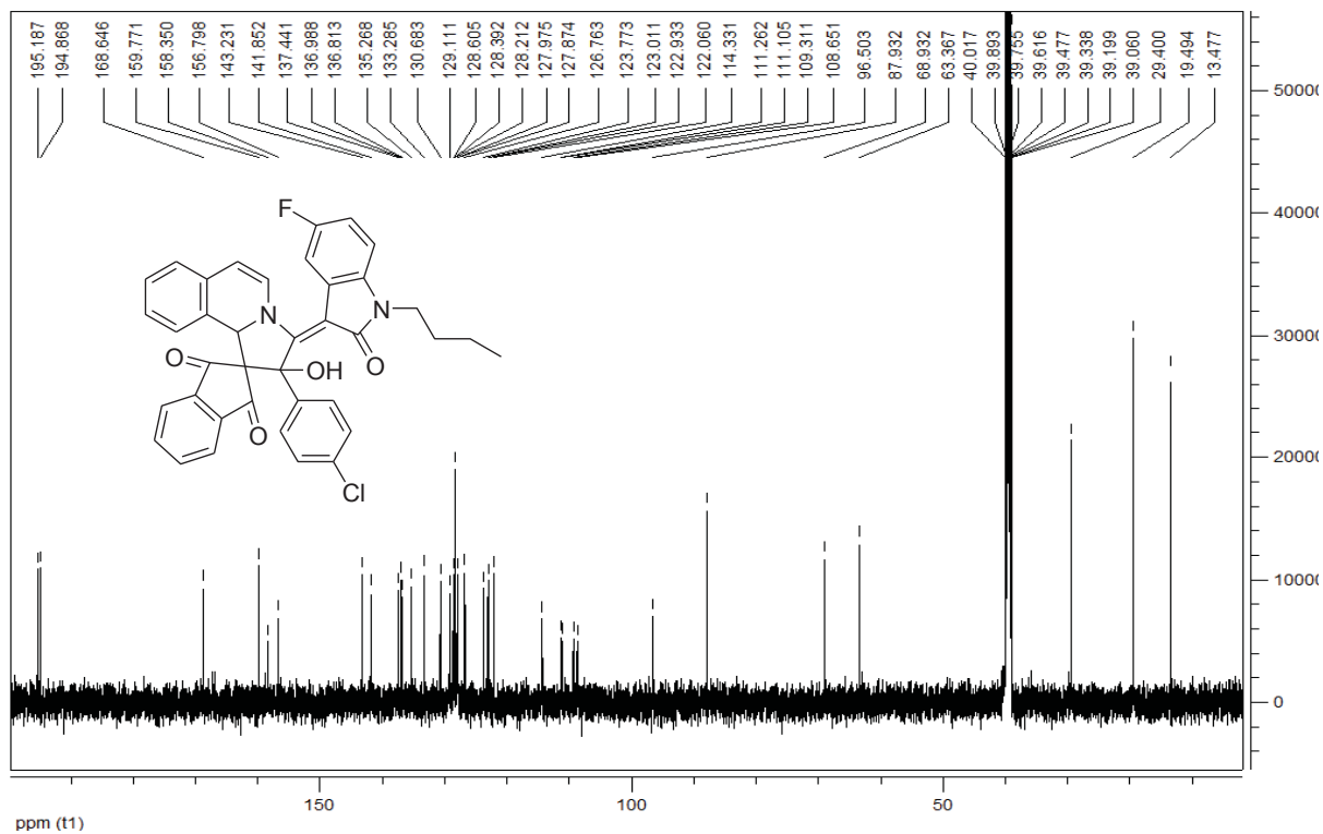
2'-acnaphthylidene spiro[indoline-2,1'-pyrrolo[2,1-a]isoquinolines] (4a)
