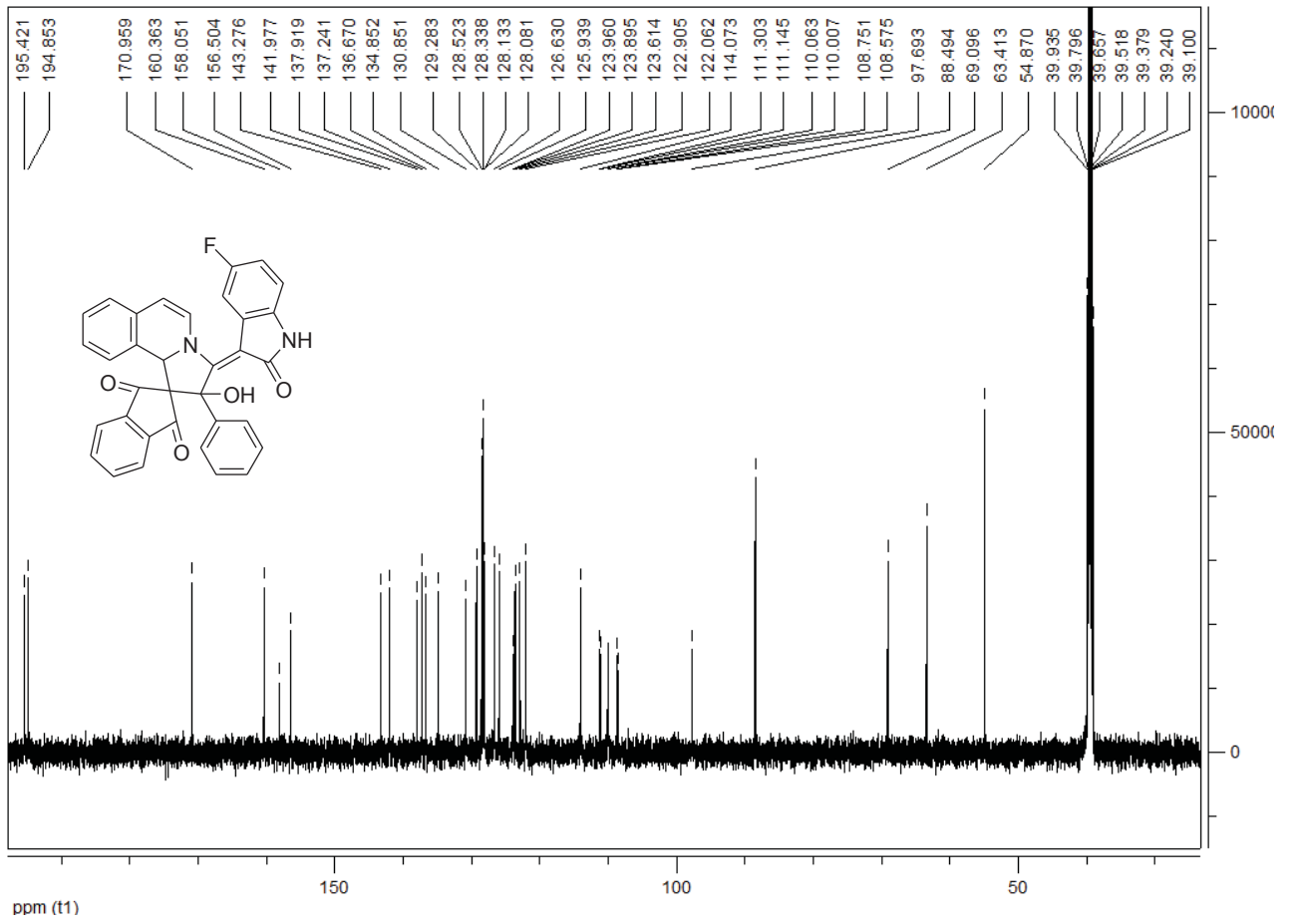
2'-Isatylidene spiro[indan-2,1'-pyrrolo[2,1-a]isoquinoline] 3d
