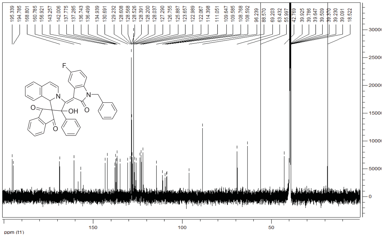
2'-Isatylidene spiro[indan-2,1'-pyrrolo[2,1-a]isoquinoline] 3m
