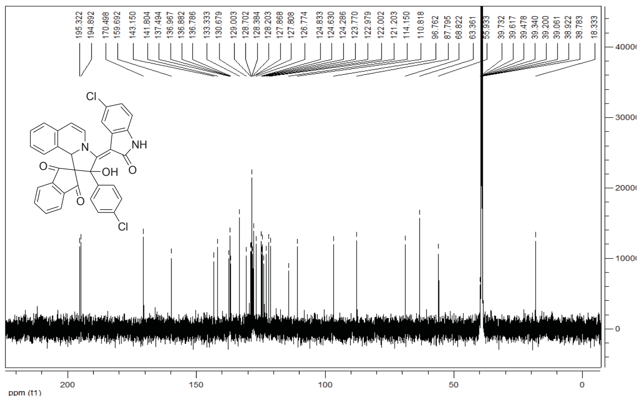
2'-Isatylidene spiro[indan-2,1'-pyrrolo[2,1-a]isoquinoline] 3i
