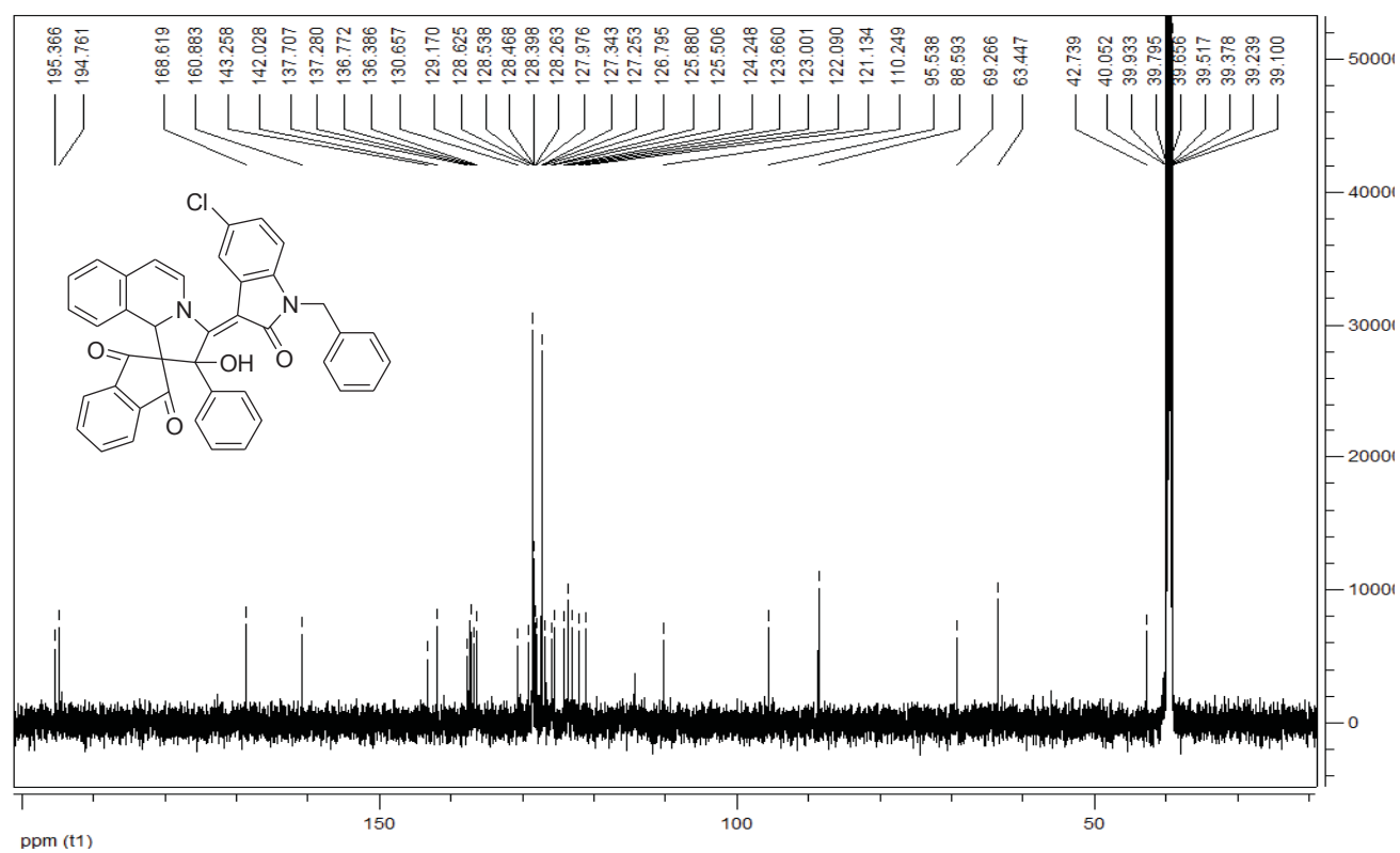
2'-Isatylidene spiro[indan-2,1'-pyrrolo[2,1-a]isoquinoline] 31
