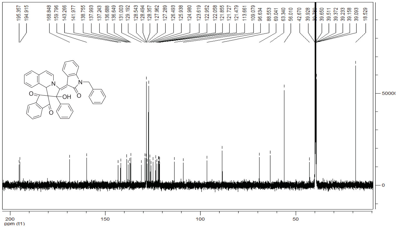
2'-Isatylidene spiro[indan-2,1'-pyrrolo[2,1-a]isoquinoline] 3j
