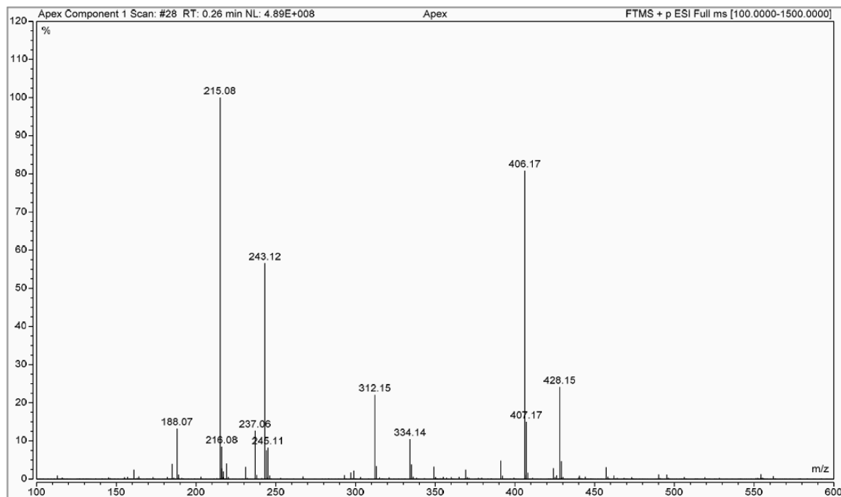
Fig. S6 MS spectrum of ML-5-Z1.
