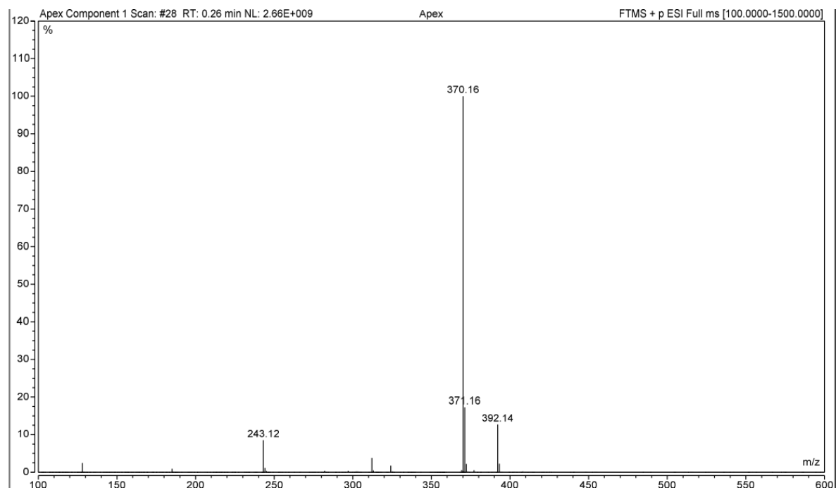
Fig. S12 MS spectrum of ML-6.
