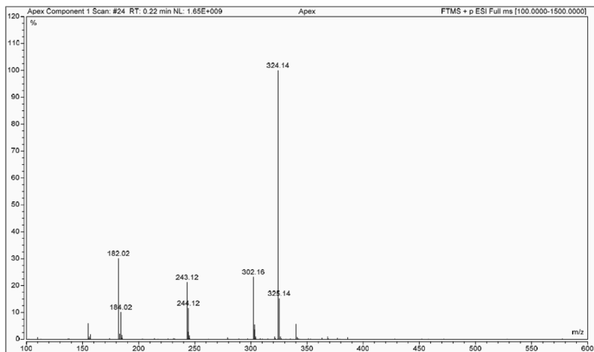
Fig. S10 MS spectrum of ML-5-Z3.
