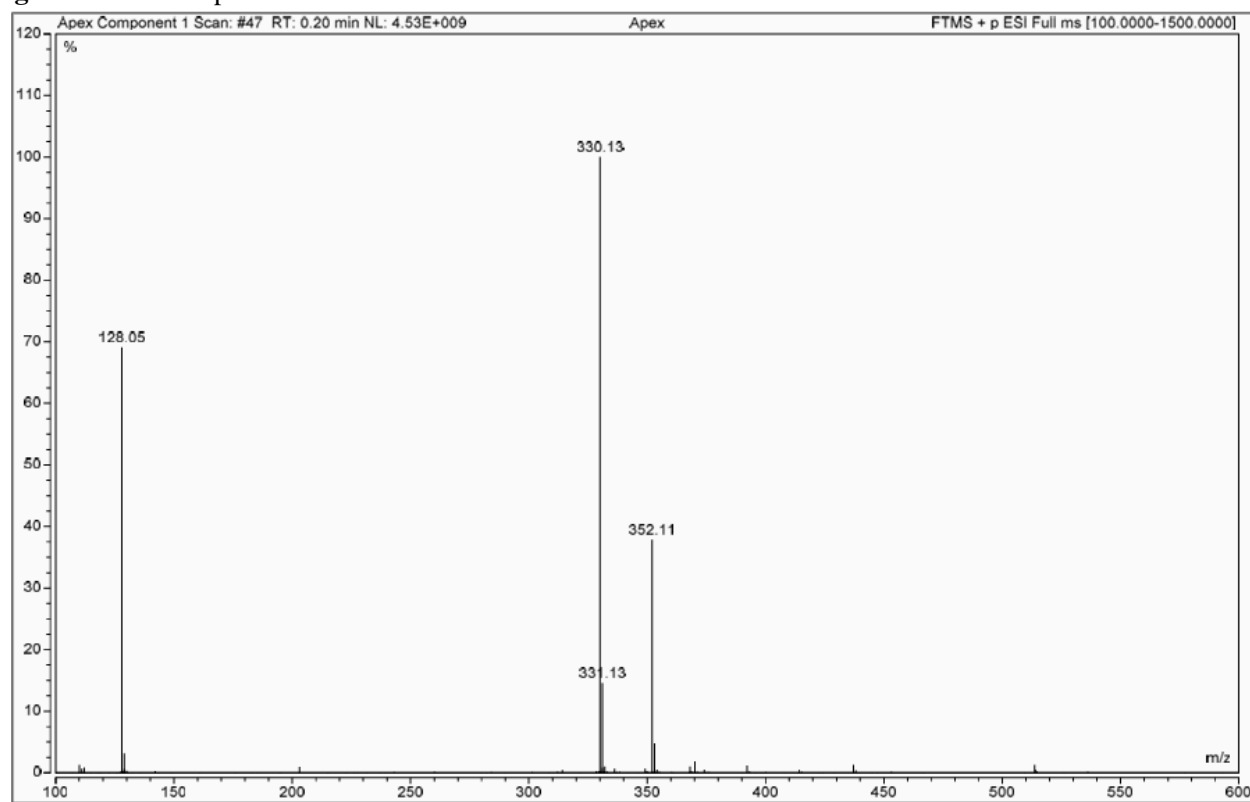
Fig. S14 MS spectrum of ML-1.
