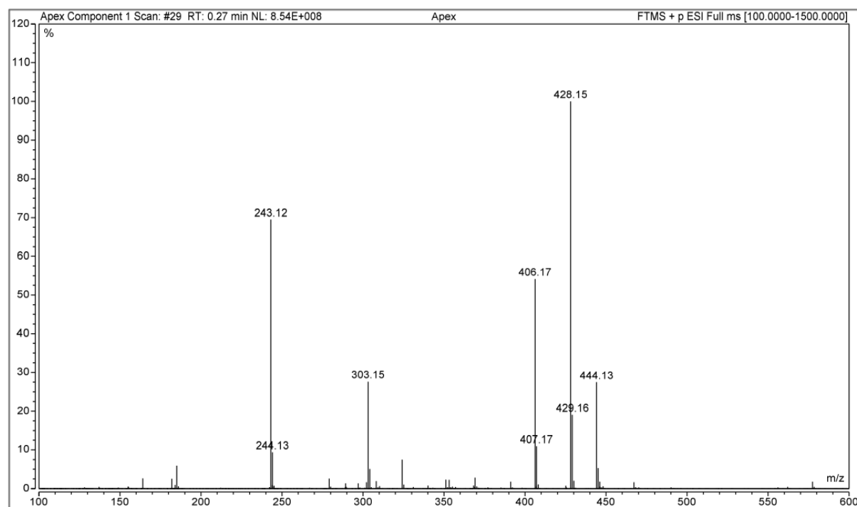
Fig. S4 MS spectrum of ML-5.
