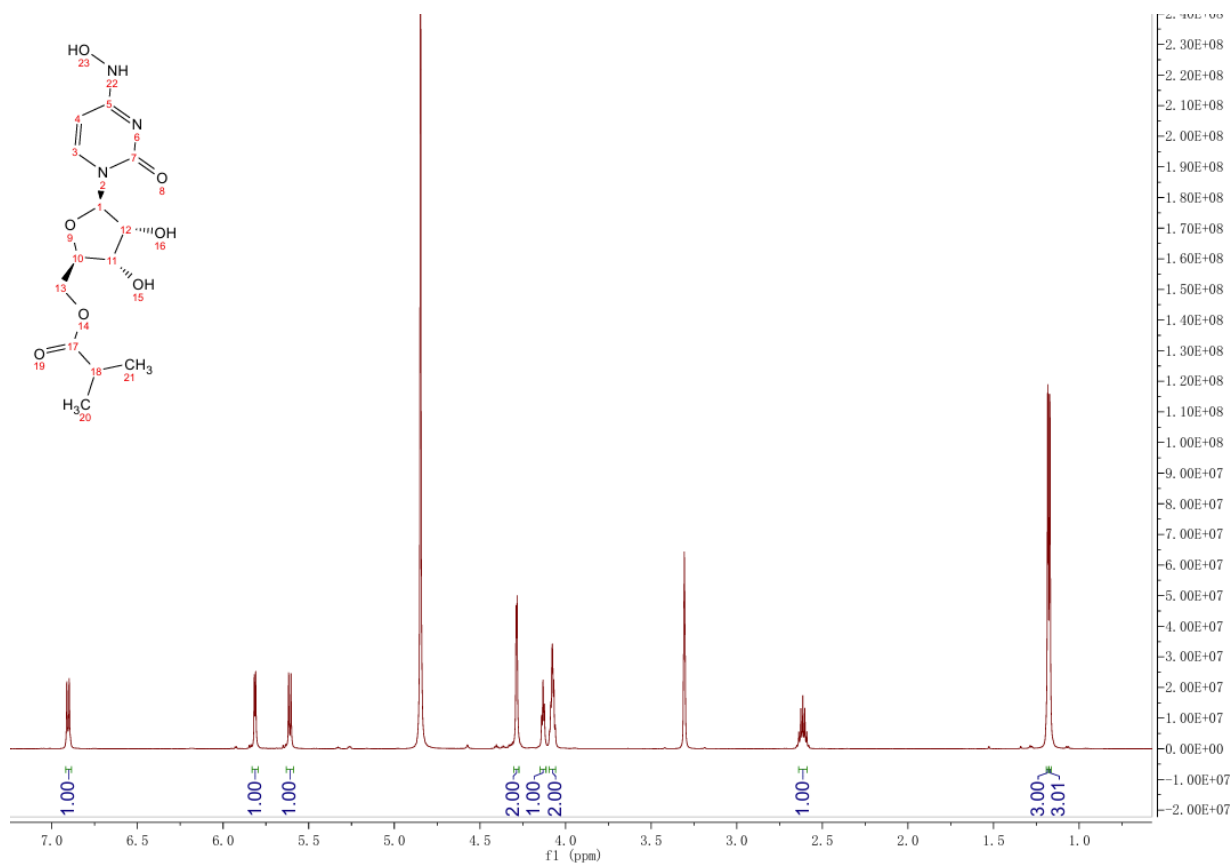
Fig. S13 1 H NMR spectrum of ML-1.
