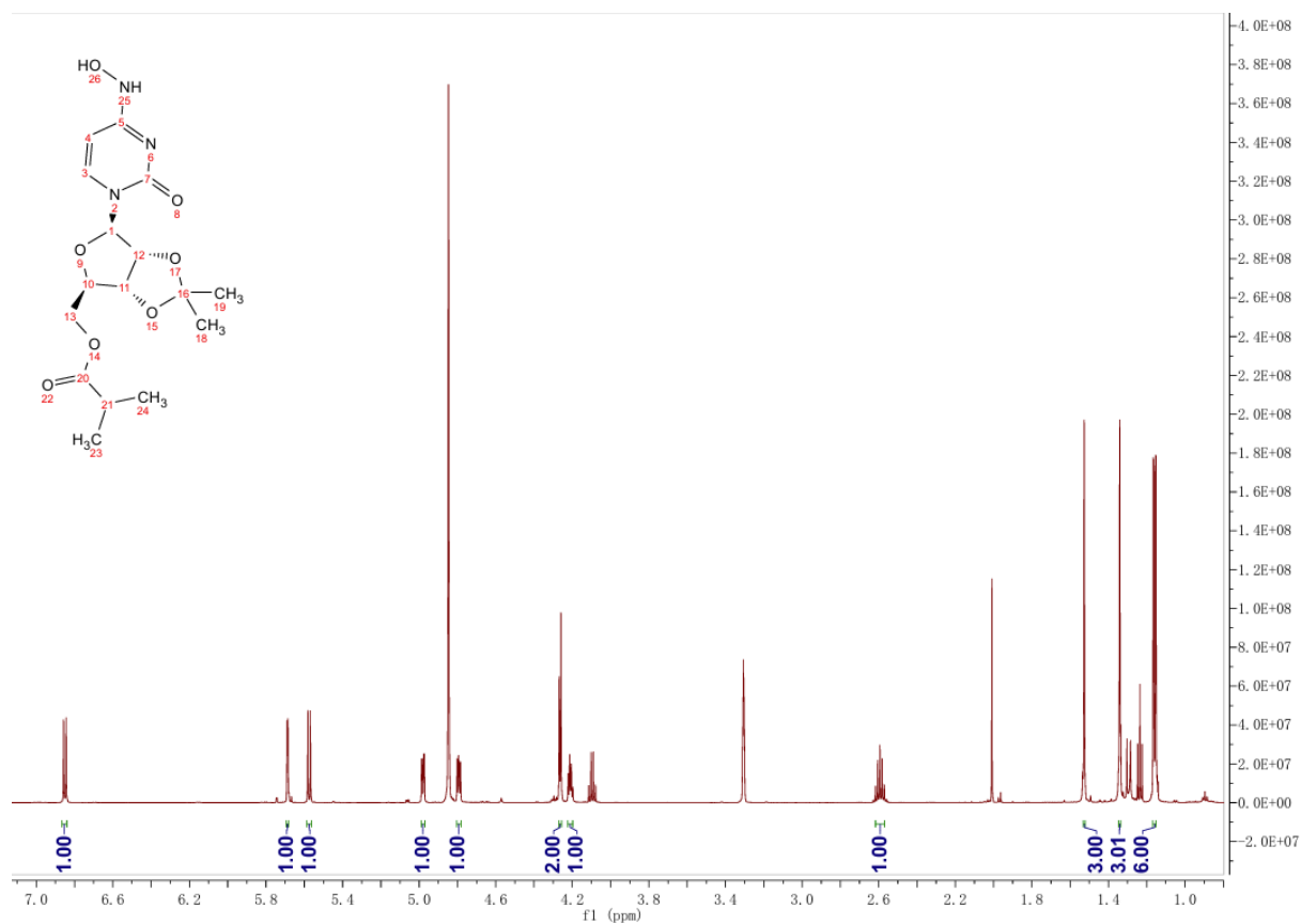
Fig. S11 1 H NMR spectrum of ML-6.
