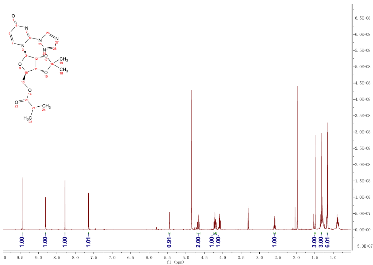
Fig. S5 1 H NMR spectrum of ML-5-Z1.
