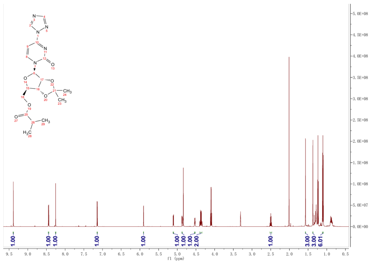
Fig. S3 1 H NMR spectrum of ML-5.
