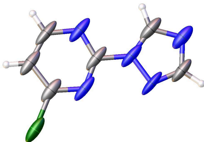
Fig. S16 X-ray of ML-5-Z3.
