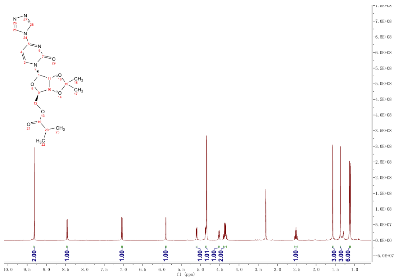
Fig. S7 1 H NMR spectrum of ML-5-Z2.
