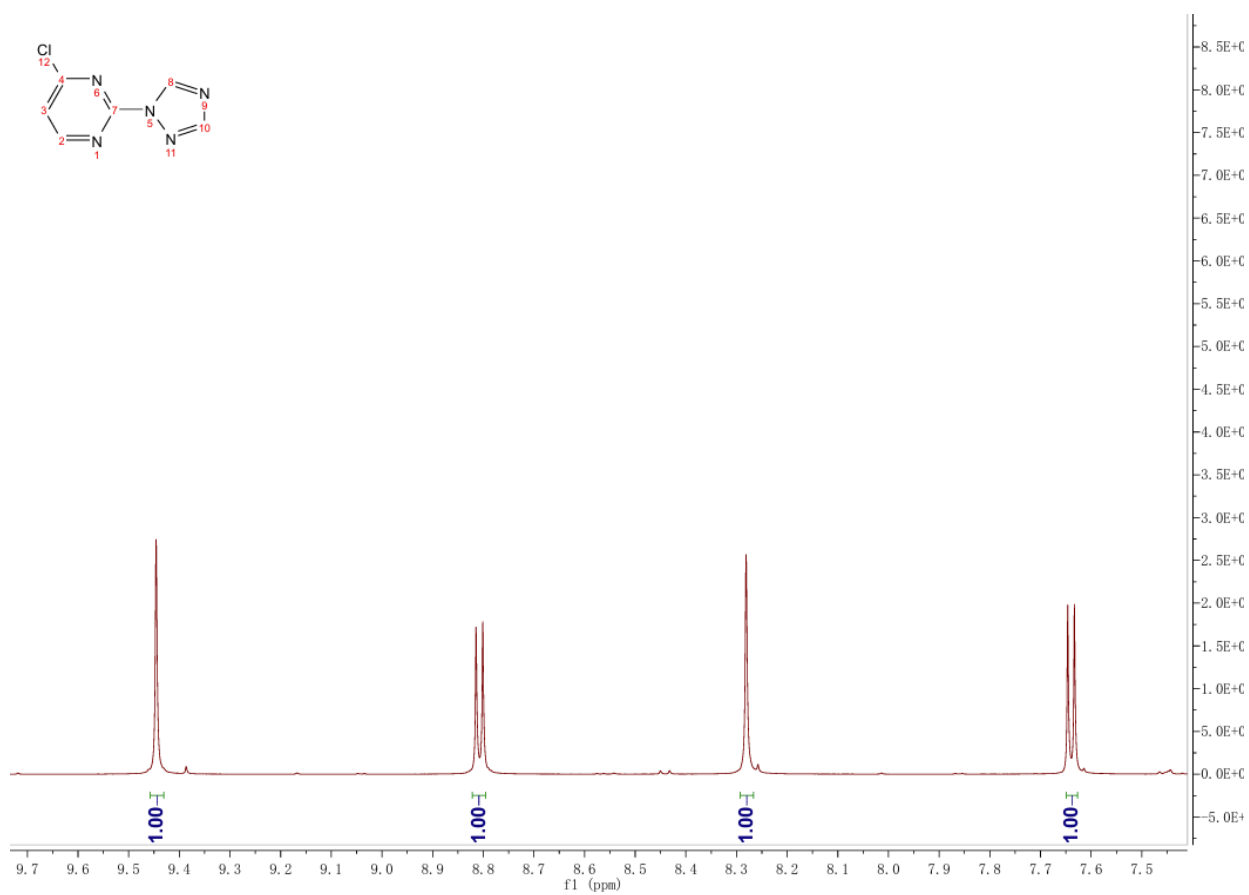
Fig. S9 ^1\text{H} NMR spectrum of ML-5-Z3.
