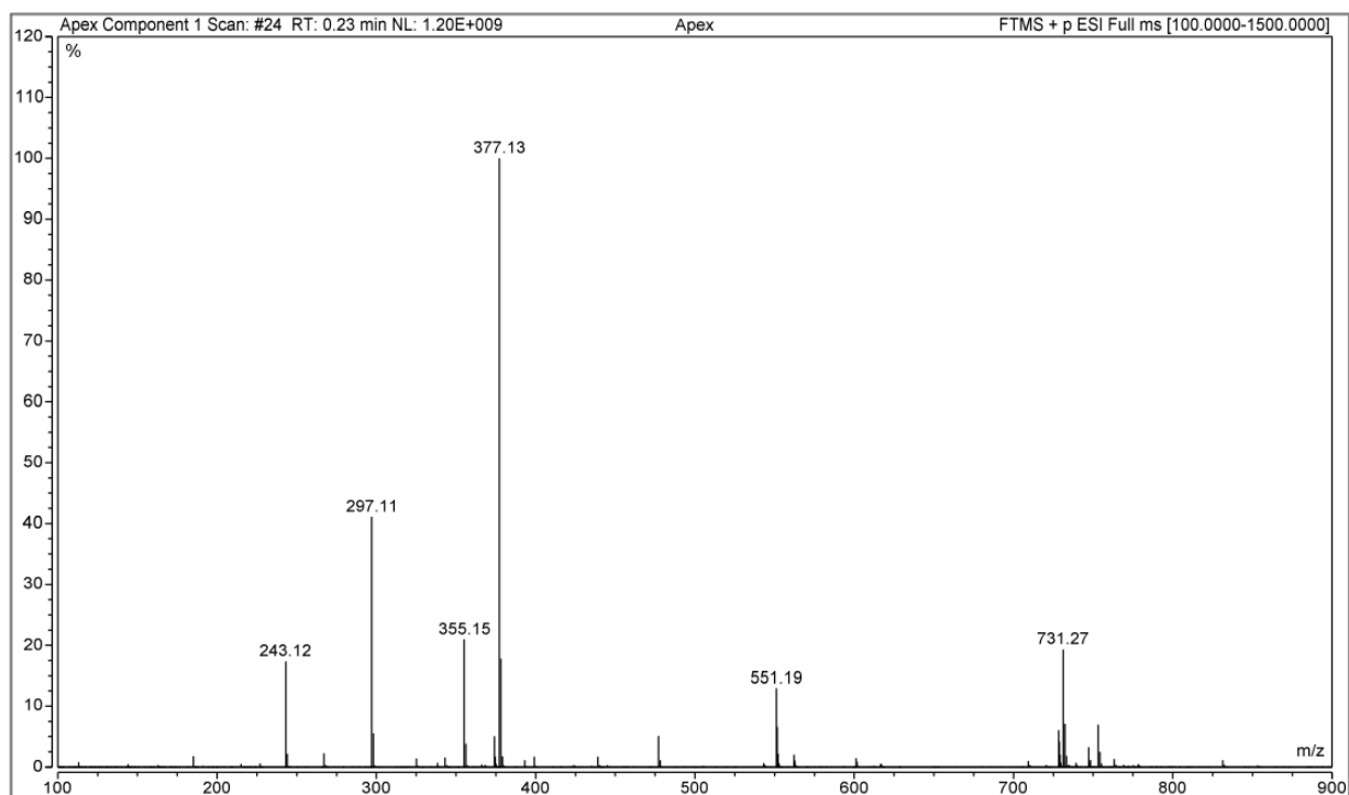
Fig. S2 MS spectrum of ML-4.
