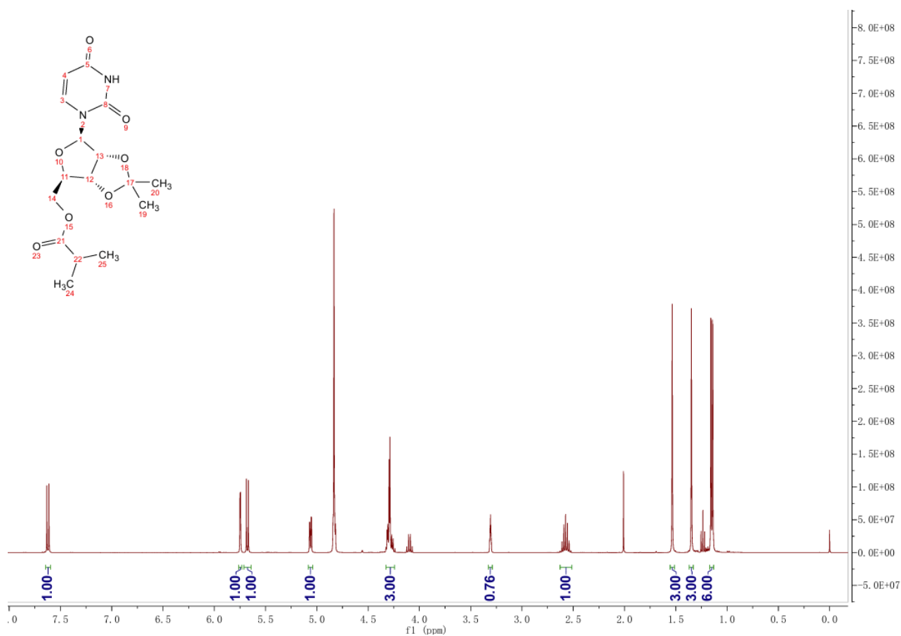
Fig. S1 1 H NMR spectrum of ML-4.
