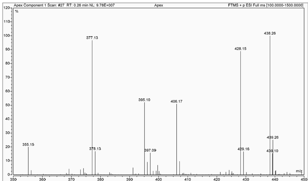
Fig. S8 MS spectrum of ML-5-Z2.
