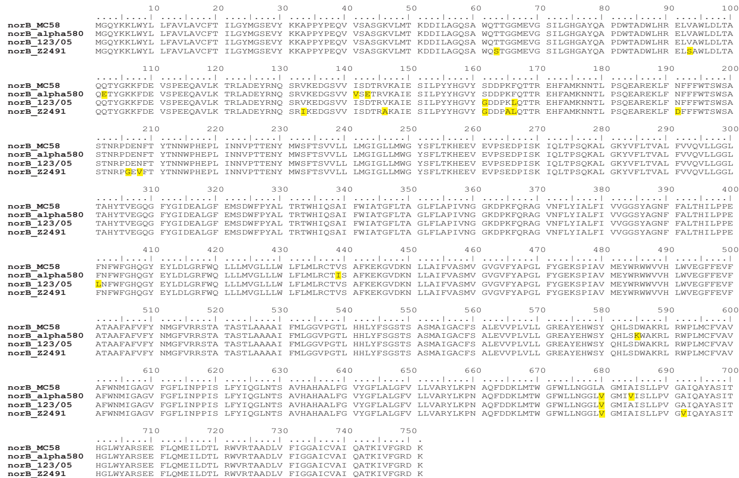
Suppl. Figure 1: Amino acid sequence alignment obtained for the protein NorB deduced from the gene sequences for the analysed N. meningitidis strain 123/05 and \alpha 580, compared with the MC58 and Z2491 nitrite oxide reductase. Colour (yellow) indicates point mutations.
