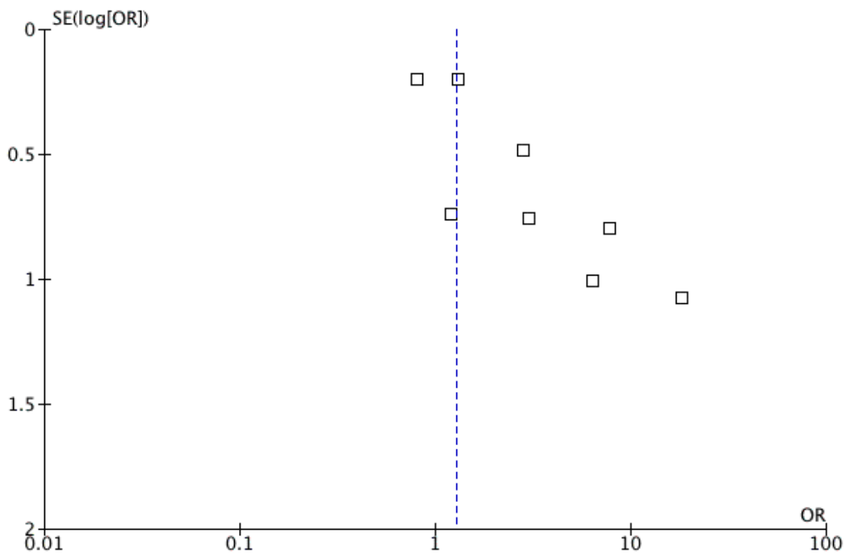
S. Figure 4. Funnel plot for studies investigating low protein Z levels in relation to venous thromboembolic diseases
