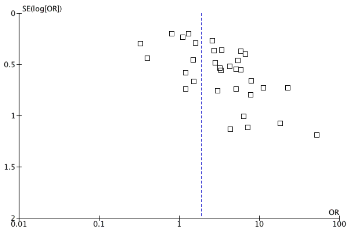
S. Figure 1. Funnel plot for studies investigating low protein Z levels in relation to vascular thrombotic diseases
