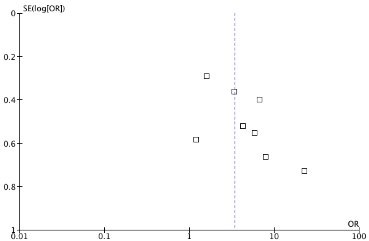
S. Figure 3. Funnel plot for studies investigating low protein Z levels in relation to pregnancy complications
