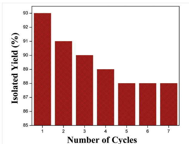
Figure 5 Recyclability test of the SrGO catalyst
