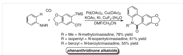
Scheme 52 Synthesis of N-methylcrinasiadine, N-isopentylcrinasiadine, and N-benzylcrinasiadine
