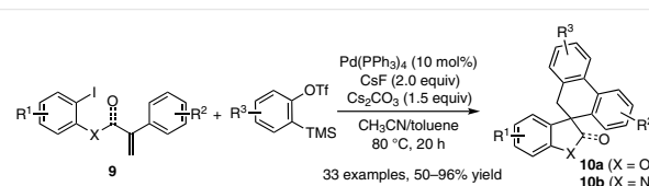
Scheme 6 Pd-catalyzed spirocyclization
