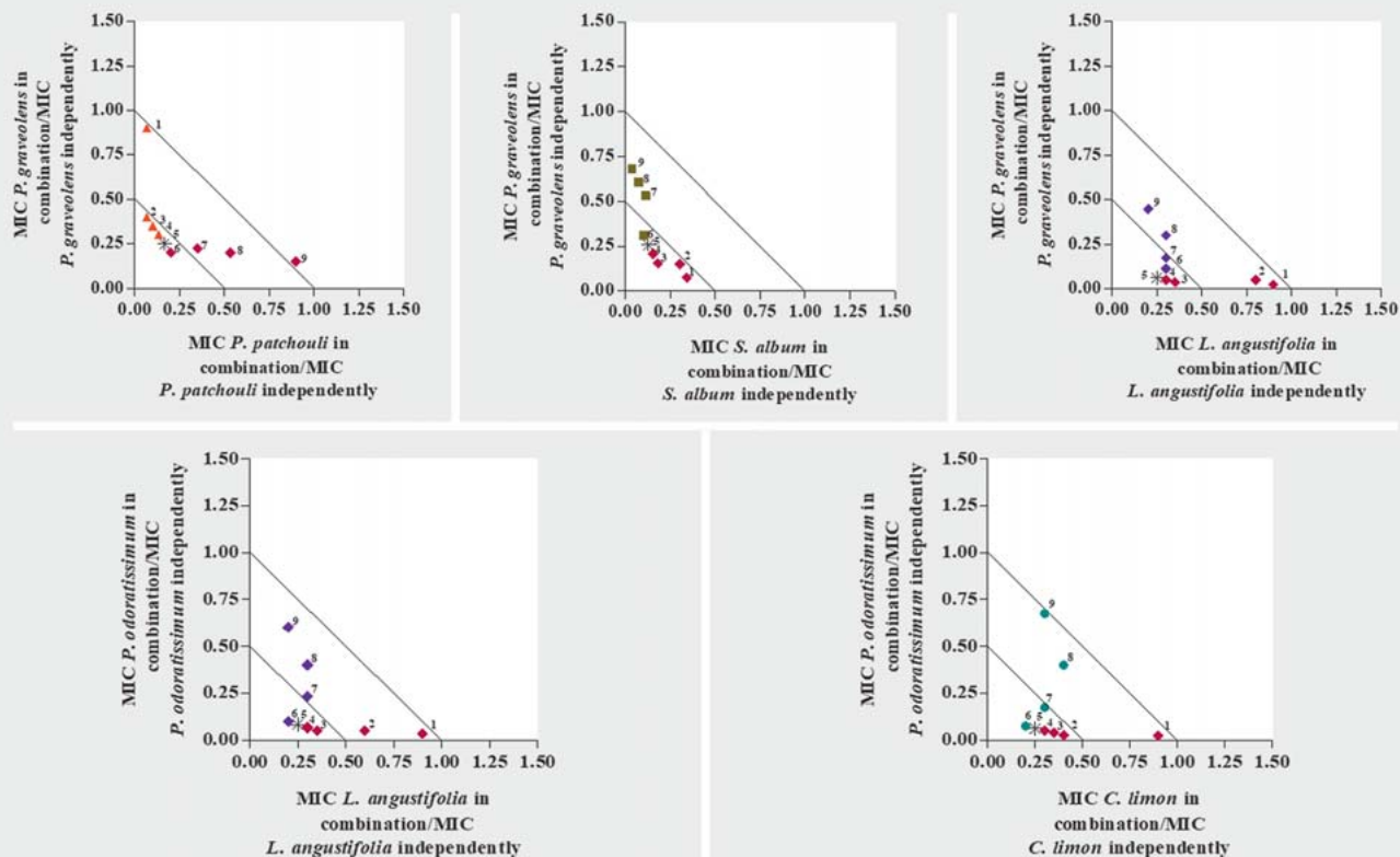
► Fig. 3 Isobologram representations of essential oils in combination containing Pelargonium spp. against B. epidermidis (DSM 20660). ♦ Pelargonium spp., ■ S. album , ◆ L. angustifolia , ● C. limon , and ▲ P. patchouli in majority volume. * Equal volume of each essential oil. Points 1–9 (► Table 5 ) provide exact concentrations of the essential oils.
